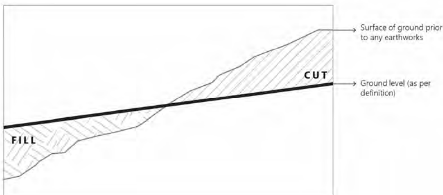
Figure 1.4.1Y: Ground level following earthworks completion where earthworks were assessed as part of an approved subdivision or mining activity
