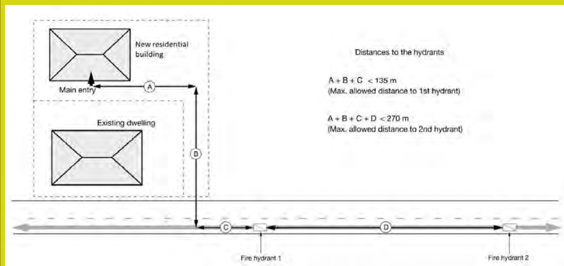
Figure 9.3.3A: Distances to fire hydrants {Change PHS1}
