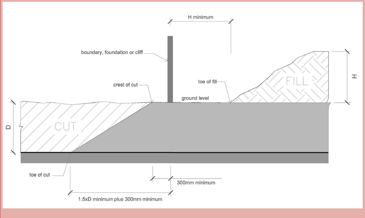
Figure 8A.5.4A: Unsupported cut and fill (elevation view)
