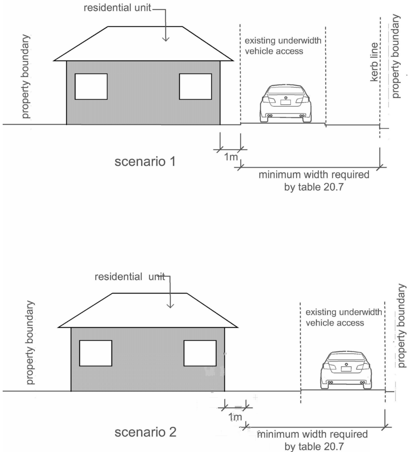
Figure 6B.5 Minimum separation distance between new residential unit and existing under-width vehicle access: possible scenarios {Variation 1 amendment - Figure 6B.5 Minimum separation distance between new residential building and existing under-width driveway: possible scenarios}
