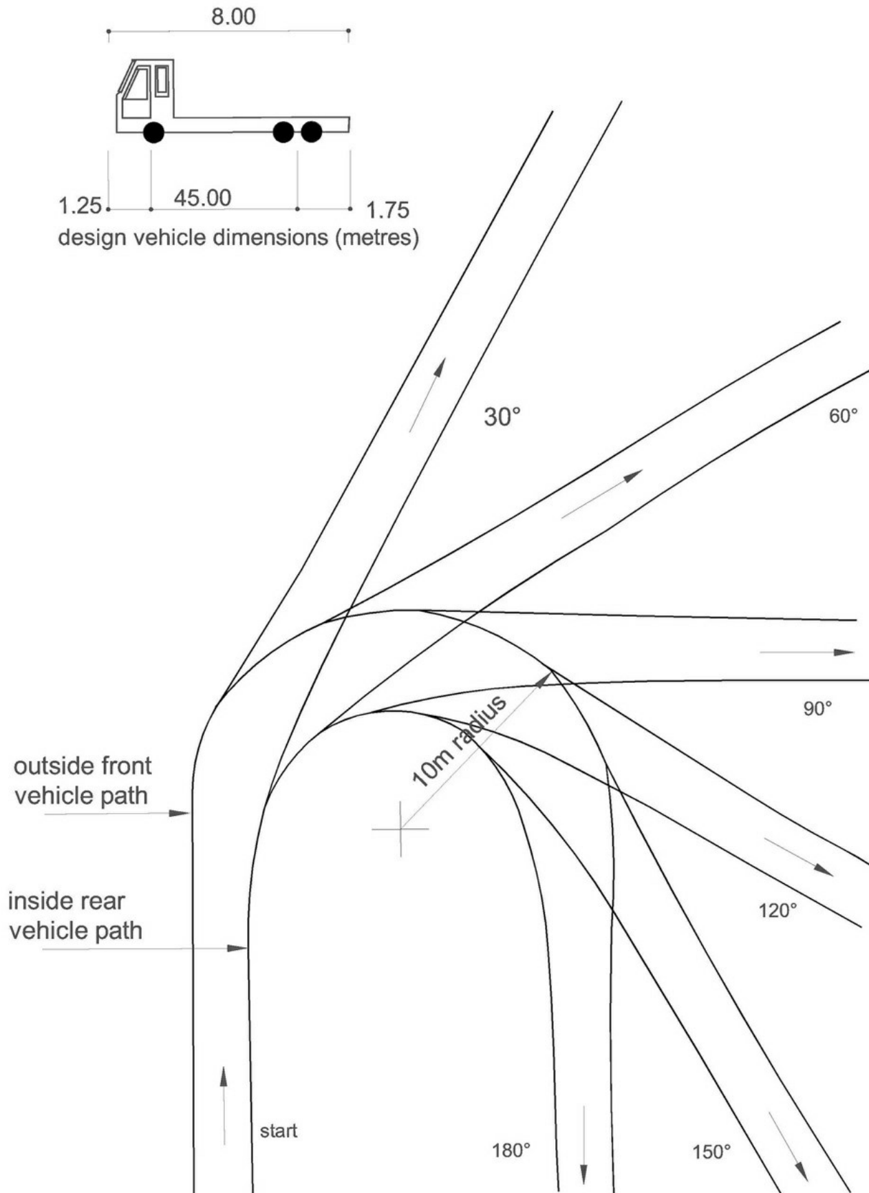
Figure 6B.10 8m rigid truck turning circle {Variation 1 amendment}
