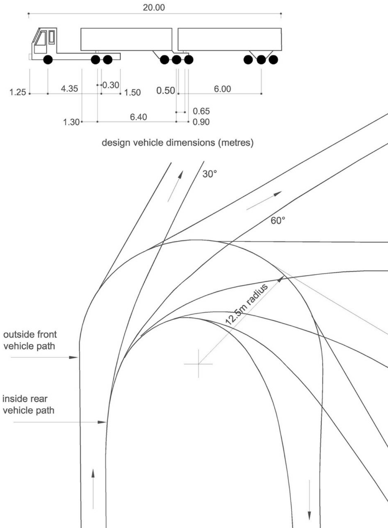
Figure 6B.12 Coach turning circle {Variation 1 amendment}
