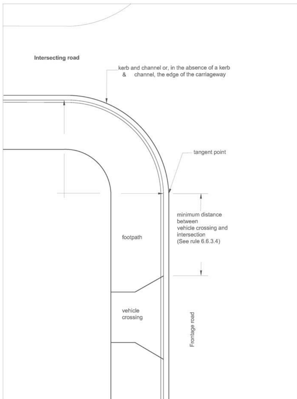
Figure 6B.17 Method to determine minimum sight distance between vehicle crossing and intersection {Variation 1 amendment - Figure 6B.17 Method to determine minimum distance between vehicle crossing and intersection}
