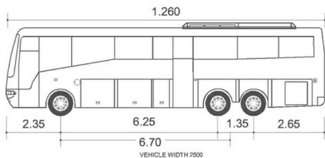
DESIGN VEHICLE DIMENSIONS (metres)
