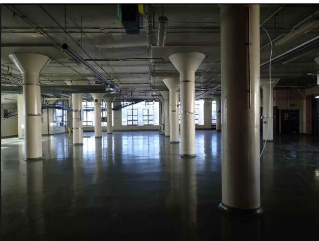
Figure C-105. Photograph looking east at the second floor of the biscuit and dispatch building (Block 5C)
