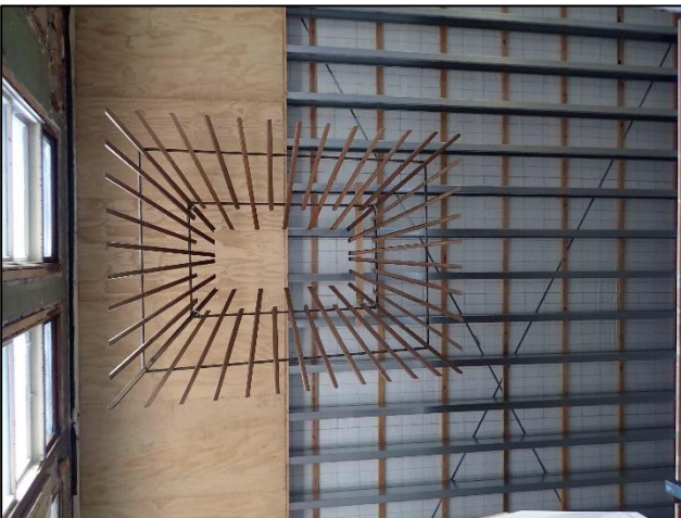
Figure C-12. Photograph showing the suspended screen visible in the 1966 plans above the stairwell to the second floor.
