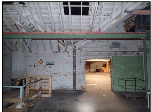
Figure C-50. Photograph looking north at interior of Cadbury World building showing steel framing added to roof structure and steel columns. Note earlier skylights have been covered.
