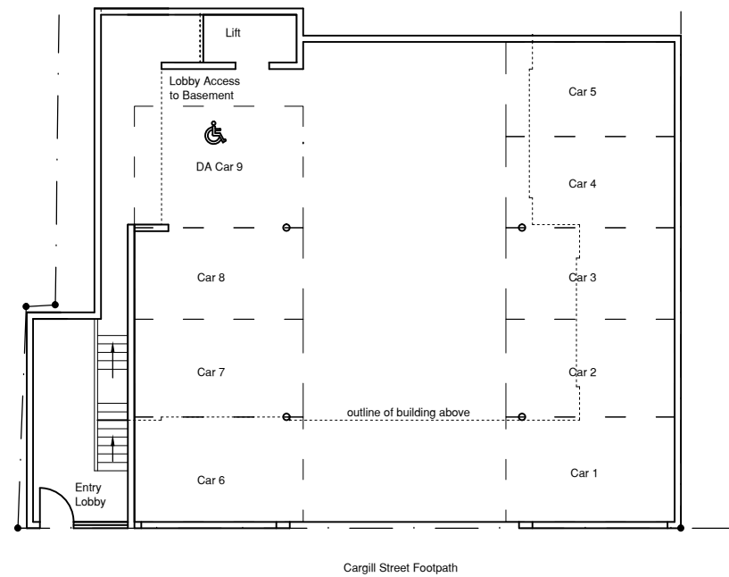
STREET LEVEL FRONT YARD & BASEMENT LAYOUT
