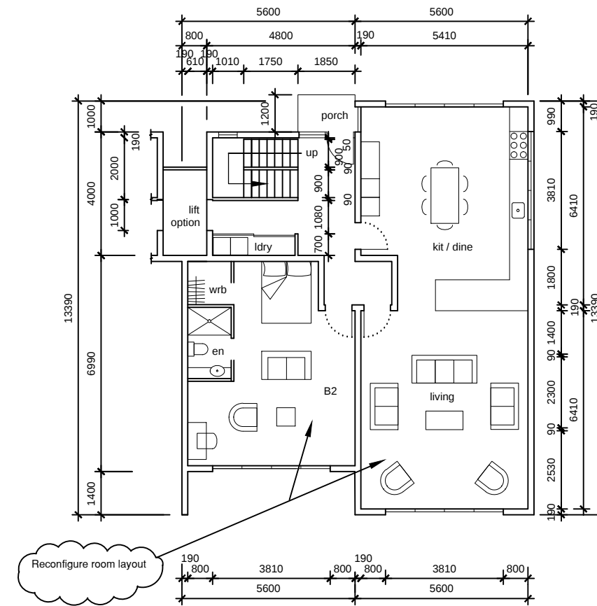
UNIT FOUR, GROUND FLOOR, PLAN LAYOUT
