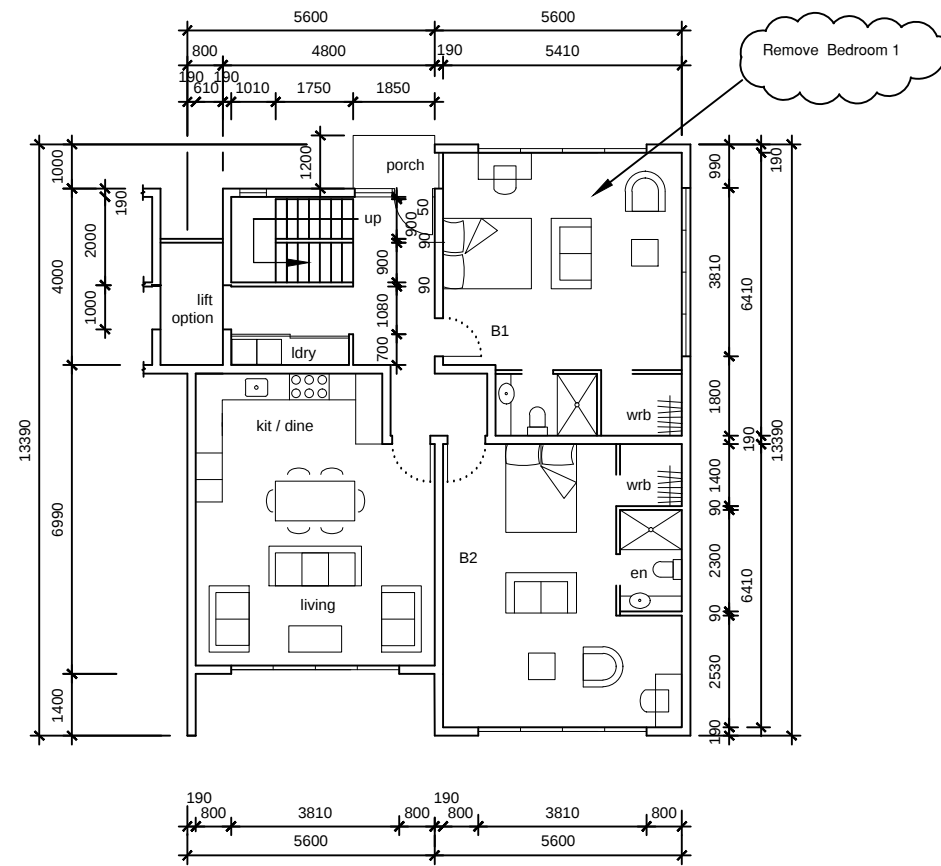
UNIT FOUR, GROUND FLOOR, PLAN LAYOUT
