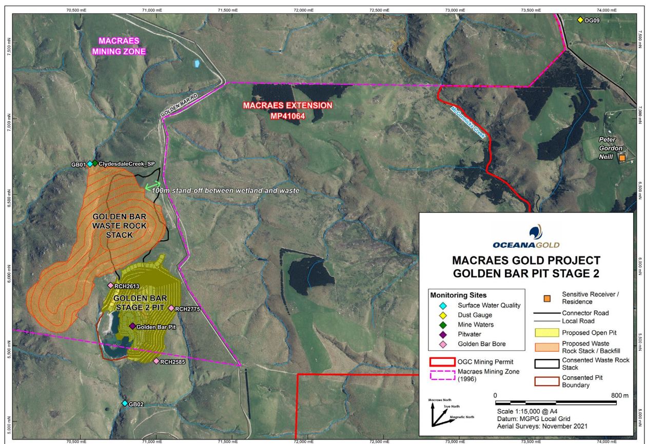
Inset 2: Plan view of the proposed Golden Bar Stage 2 cutback and WRS location. (Source OG. 2023).
