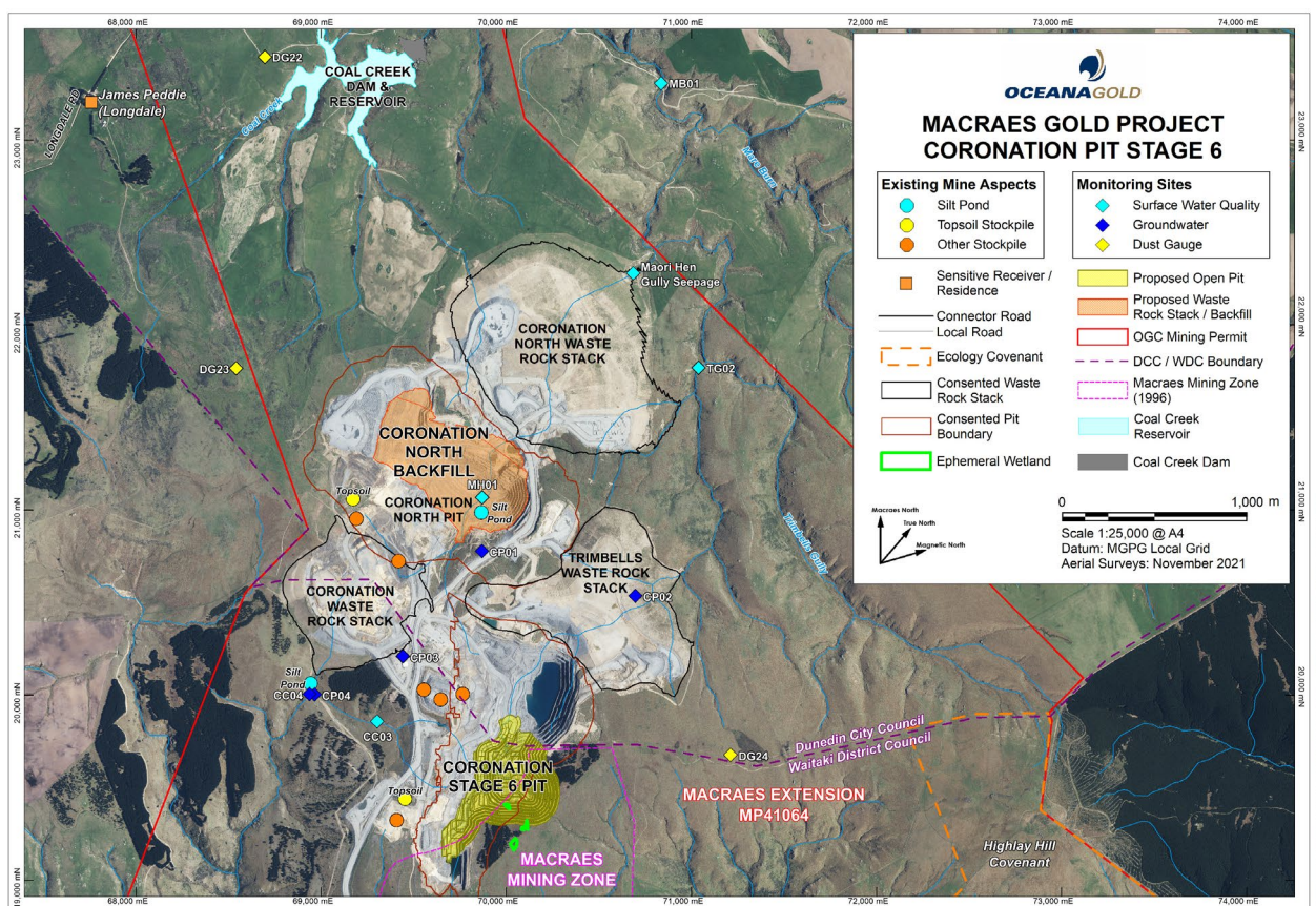
Inset 3: Plan view of the proposed Coronation Hill Stage 6 cutback and WRS location. (Source OG. 2023).
