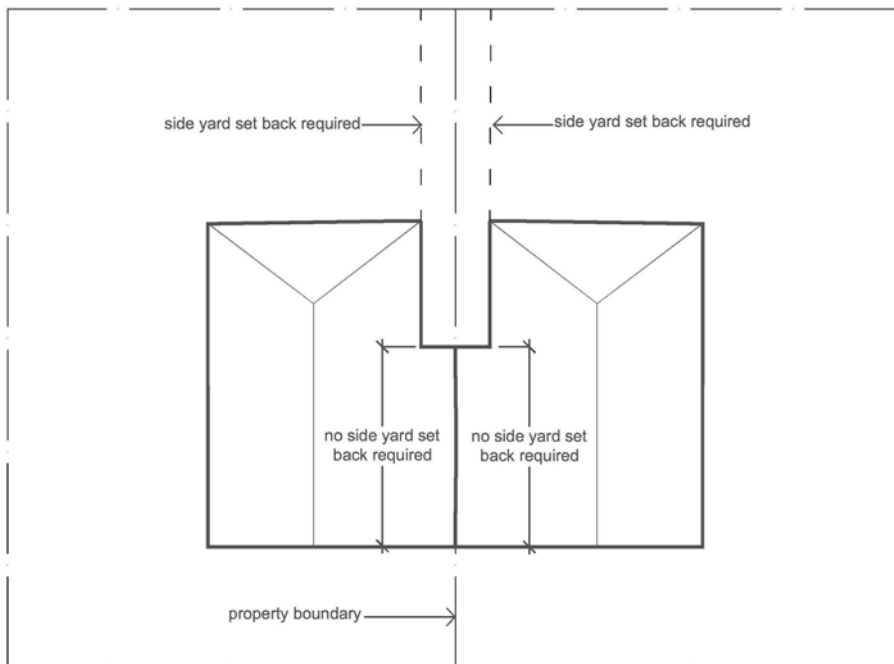
Figure 15.6.13.1B: Setbacks for buildings sharing common wall
