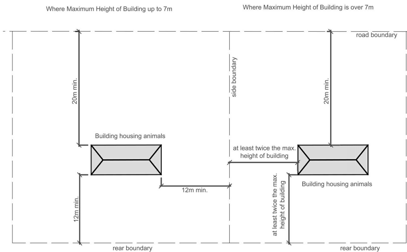
Figure 16.6.10.1B: Setbacks for non-residential buildings that house animals
