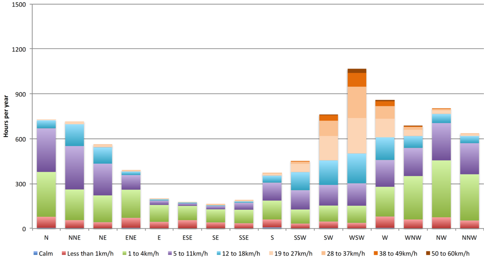
Wind Direction and Speed - Dunedin Airport
