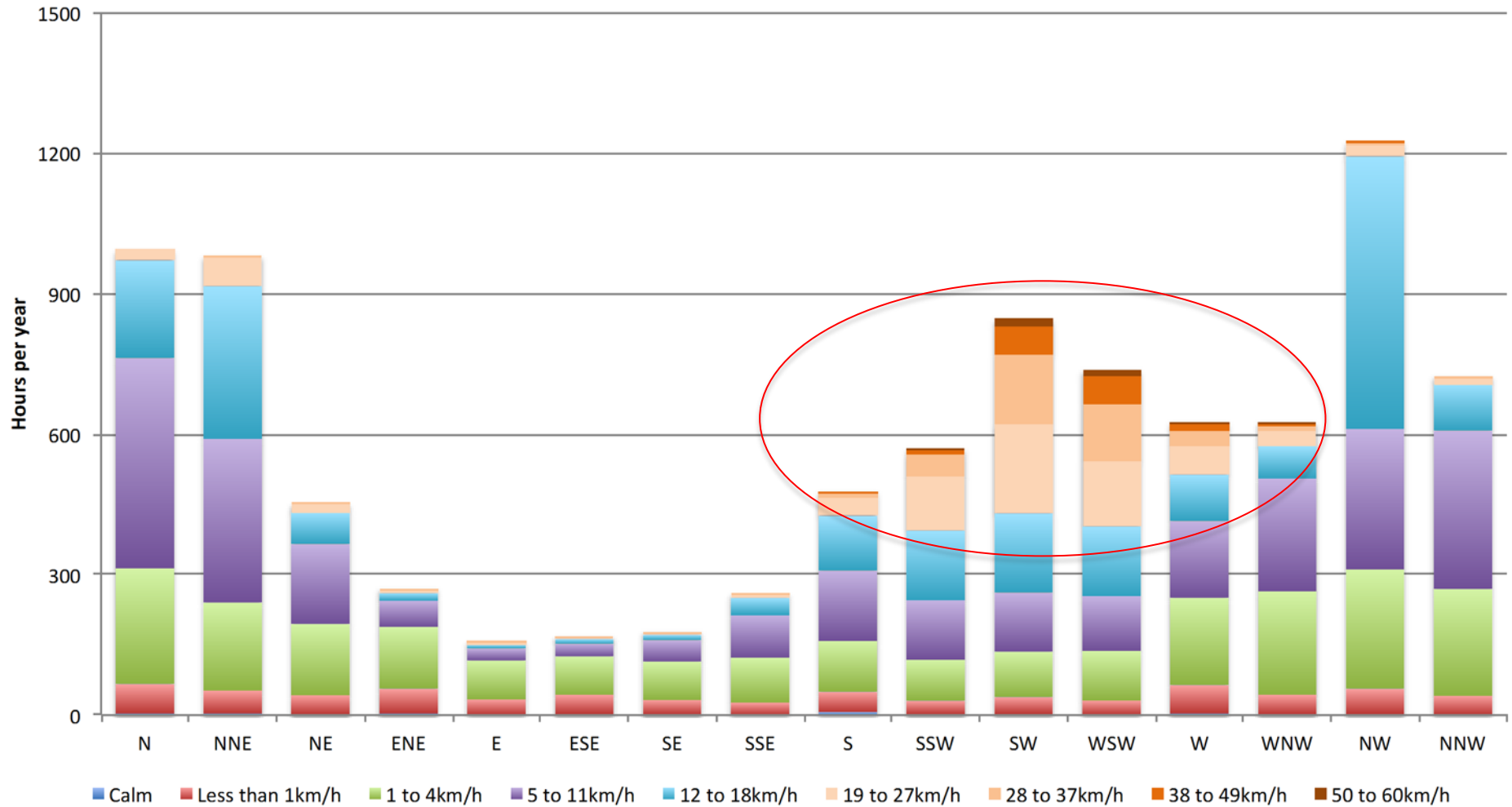
Wind Direction and Speed - The Octagon, Dunedin
