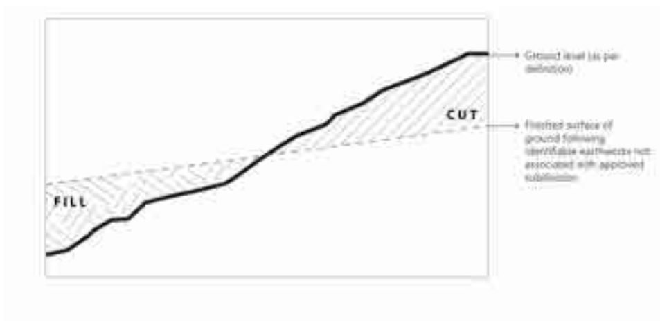
Figure 1.4.1AA: Ground level when a retaining wall/structure crosses a site boundary
