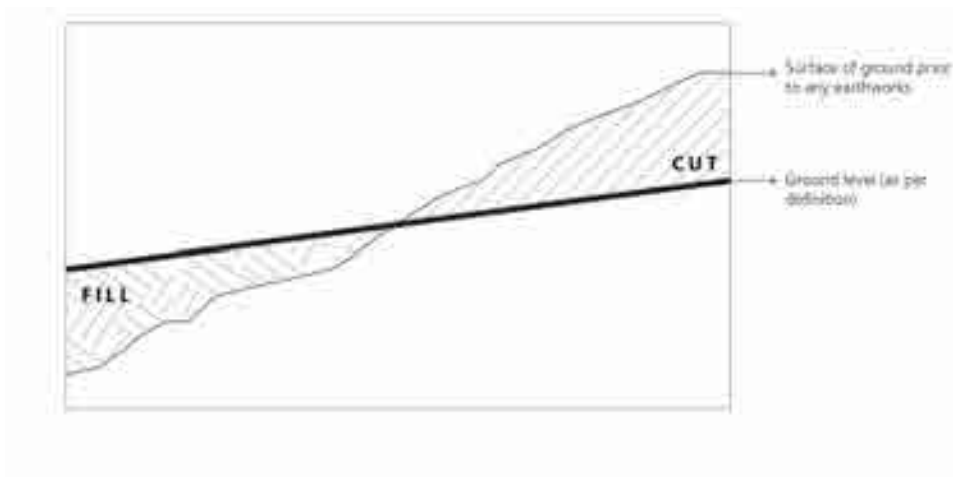
Figure 1.4.1Z: Ground level where identifiable earthworks are not associated with an approved subdivision (e.g. associated with an approved land use consent, or permitted earthworks)
