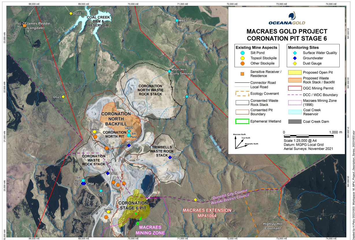
Figure 1.2 Coronation Open Pit Mining Area – Existing and Proposed.
