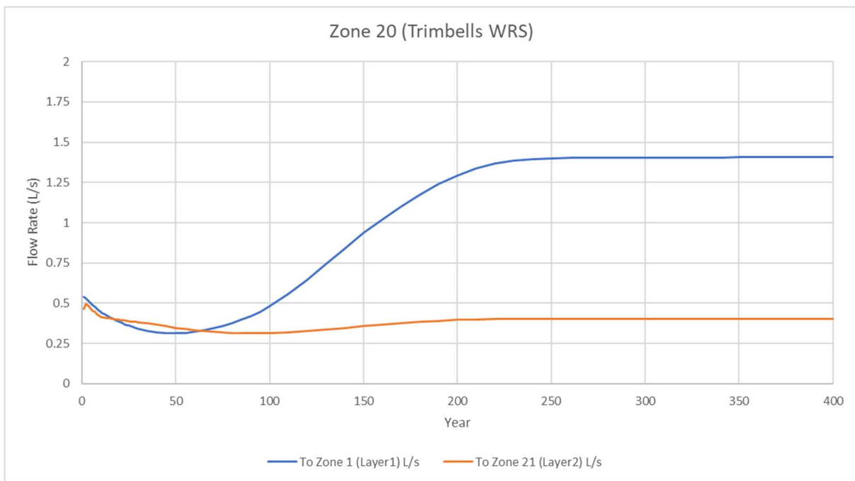
Figure 4.23 Seepage flow rate from Trimbell's WRS (zone 20) to Zone 1 (Layer 1) and Zone 21 (Layer 2)
