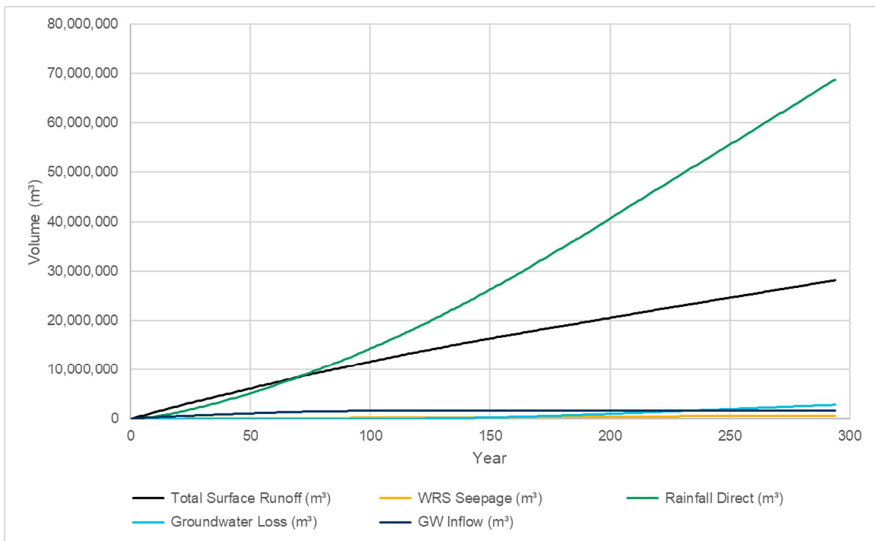
Figure 5.8 Coronation Pit Lake (CO6) cumulative water balance.
