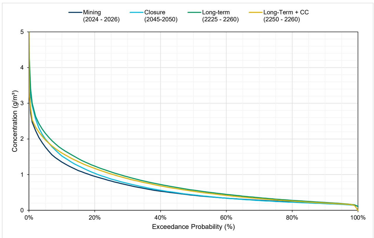
Figure 5.14 MB01 Nitrate N – Modelled probability exceedance
