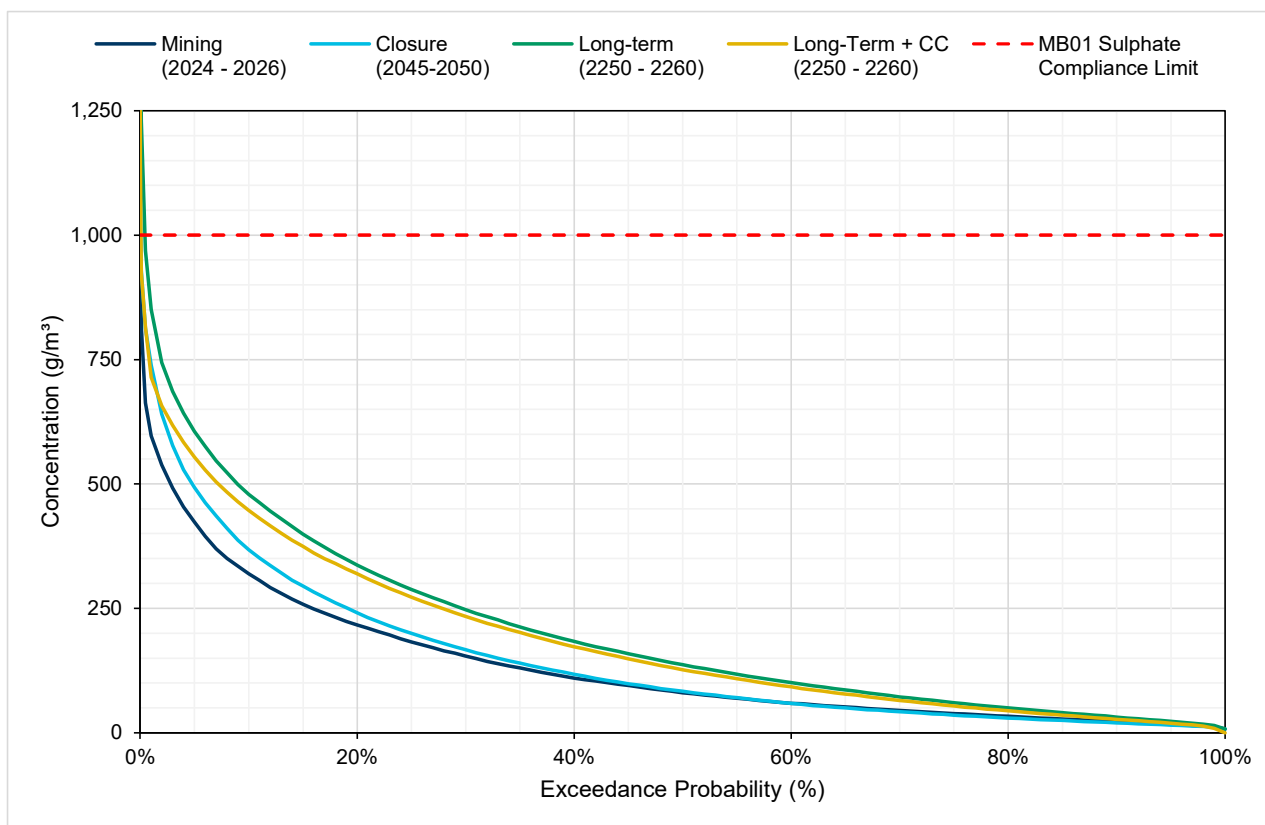
Figure 5.13 MB01 Sulphate – Modelled probability exceedance
