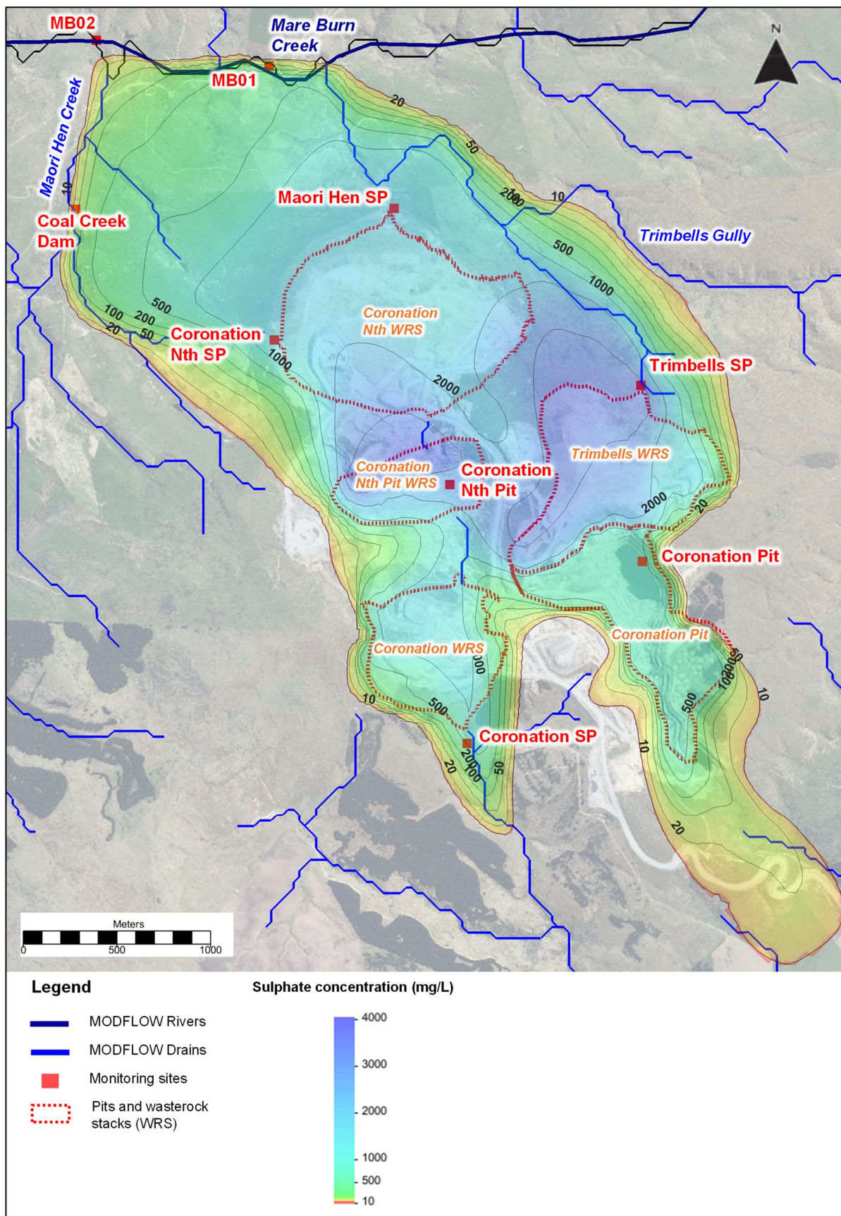
Figure 4.20 Contour plot showing plume extent in 400 years in model layer 2
