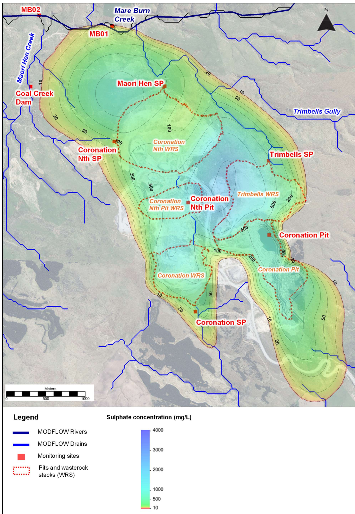
Figure 4.21 Contour plot showing plume extent in 400 years in model layer 4
