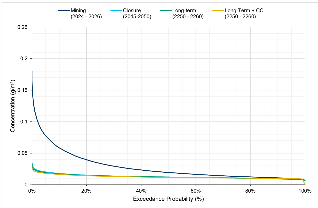
Figure 5.15 MB01 Ammoniacal N – Modelled probability exceedance
