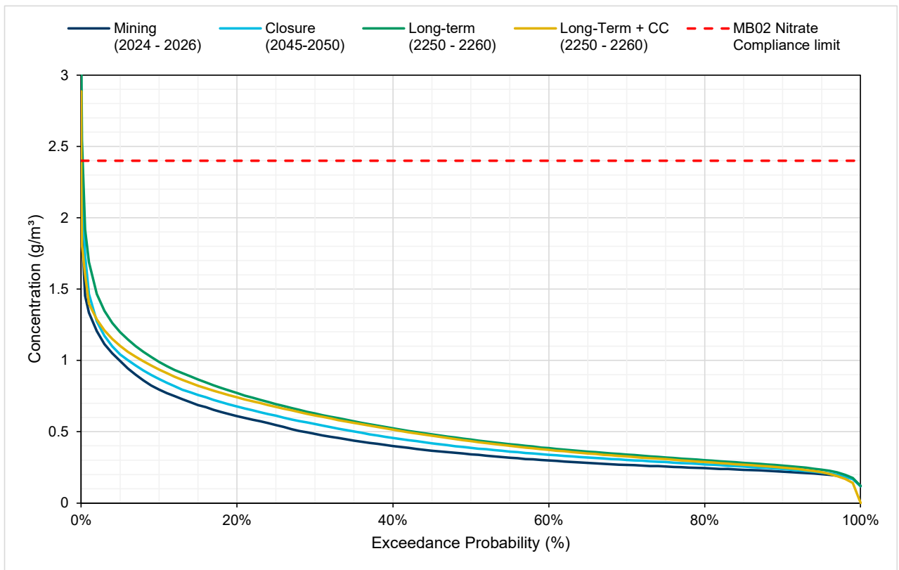
Figure 5.11 MB02 Nitrate N – Modelled probability exceedance
