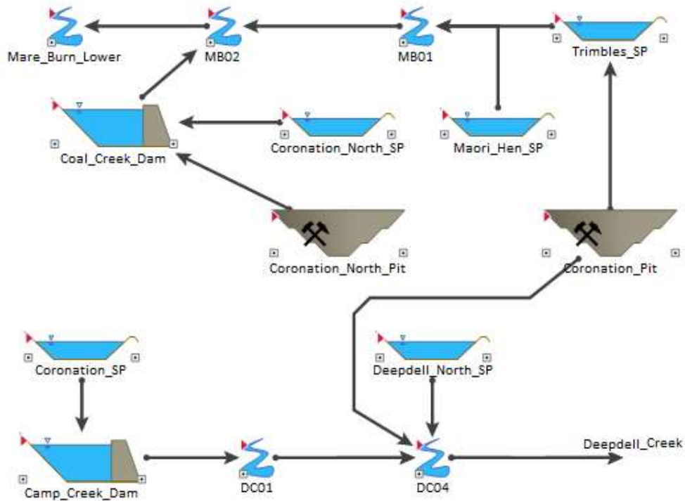
Figure 5.1 Schematic of the Coronation area elements of the Macraes Water Balance Model.
