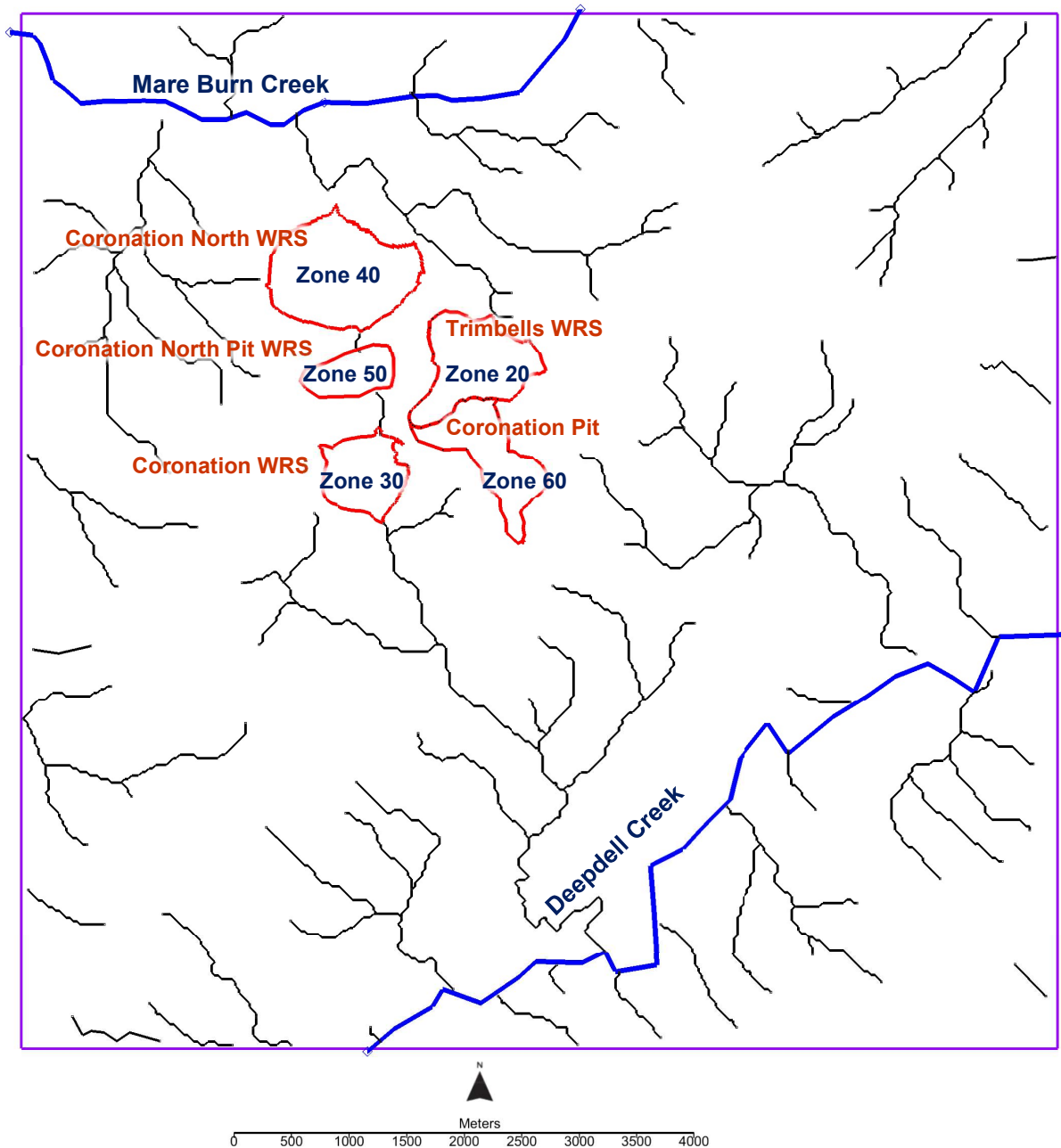
Figure 4.22 Location plan of zones to assess inflow and outflow during recovery.
