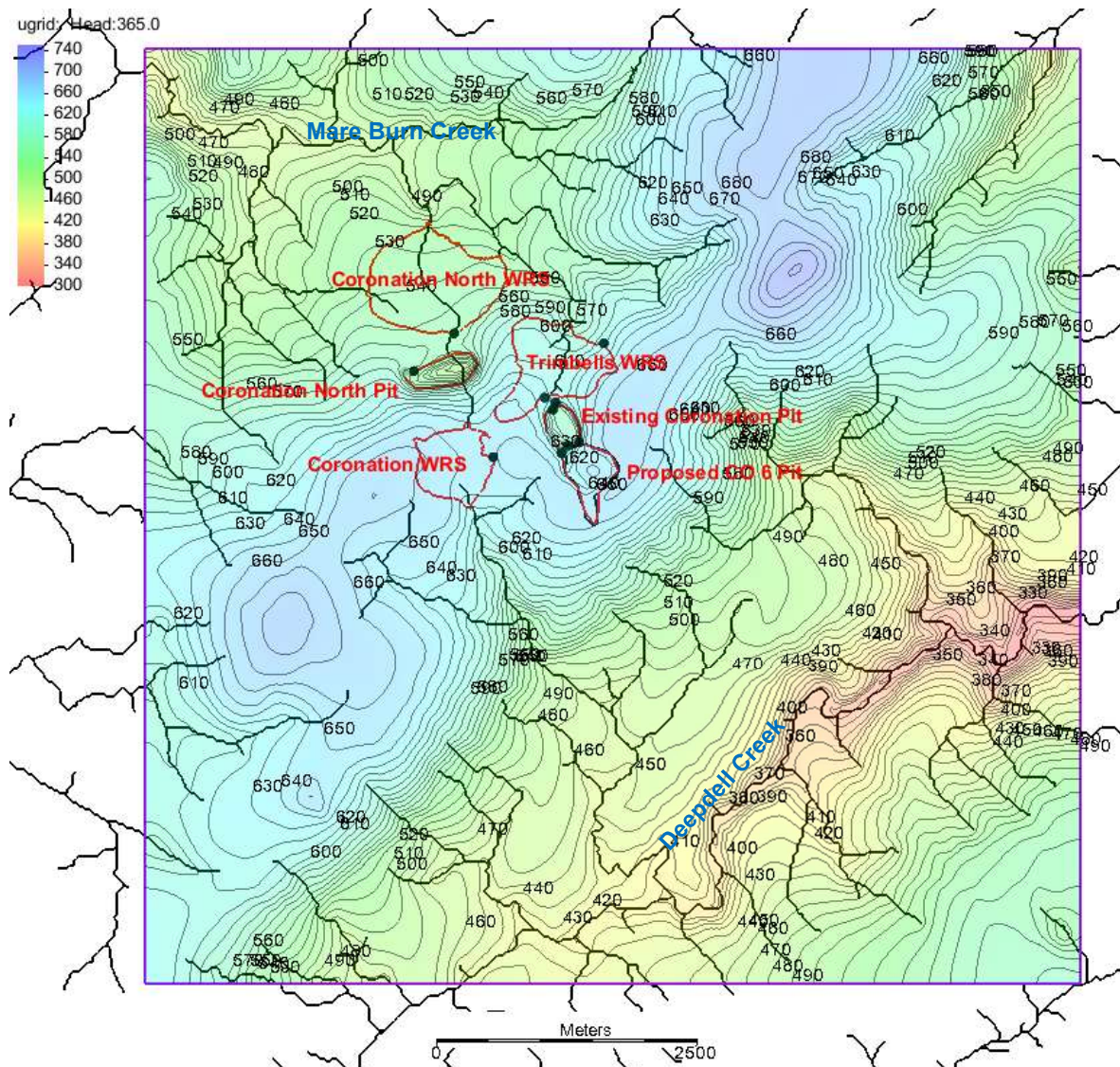
Figure 4.12 Pressure head contours at the end of dewatering (2026)
