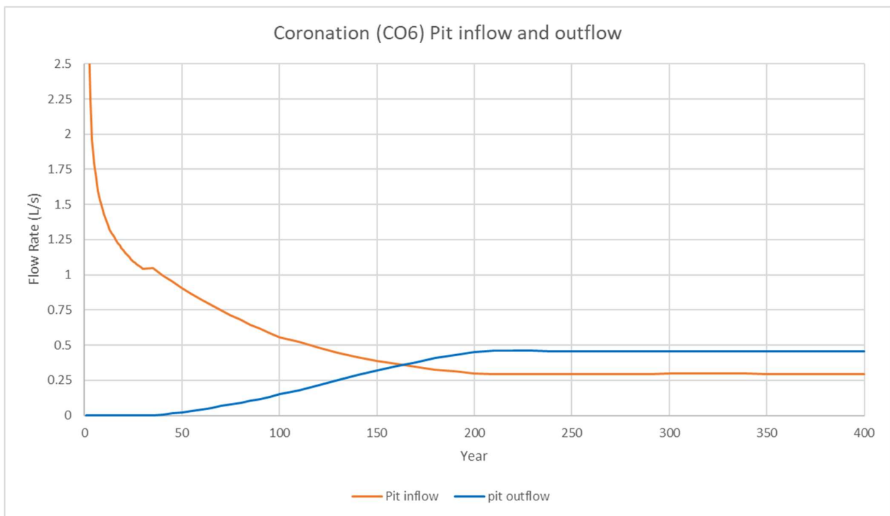
Figure 4.27 Groundwater in and outflow from the Coronation pit lake
