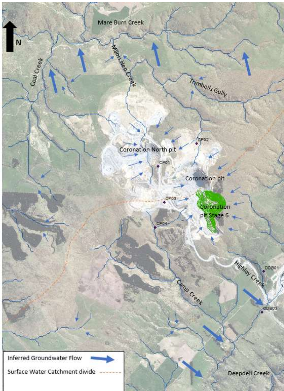
Figure 4.2 Inferred existing / proposed mining groundwater flow direction
