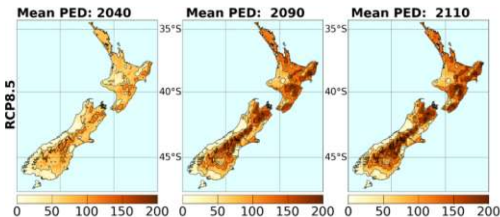
Figure 5.3 PED projections (exert from MfE 2018, Figure 55)
