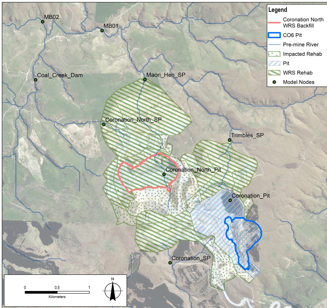
Figure 7.3 Coronation Waste Rock Stack Rehabilitated / Non-Rehabilitated Plan - Closure
