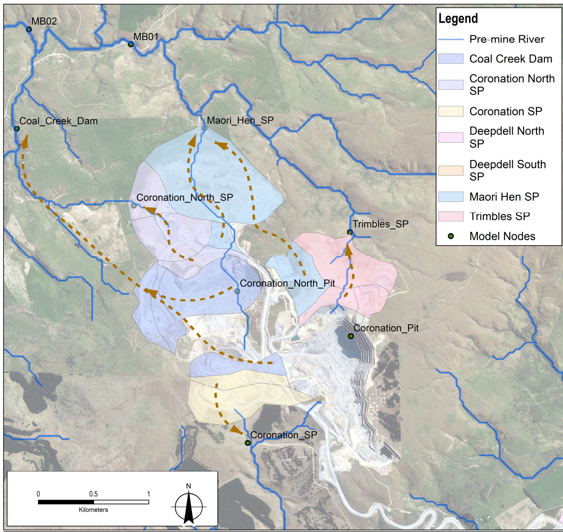
Figure 7.7 Coronation Seepage Catchment Map - Closure
