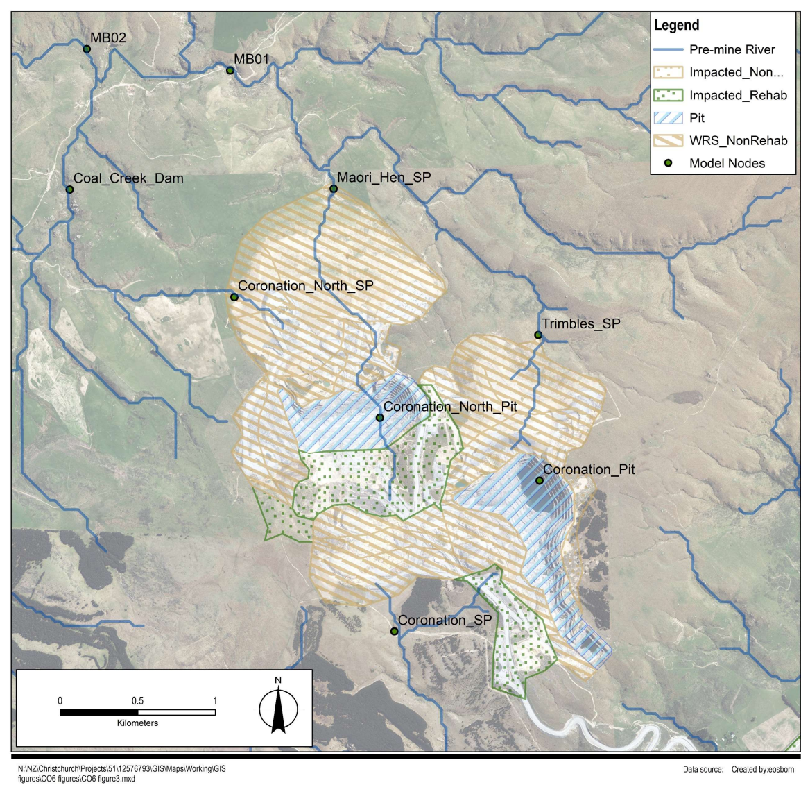
Figure 7.2 Coronation Waste Rock Stack Rehabilitated / Non-Rehabilitated Plan - Current
