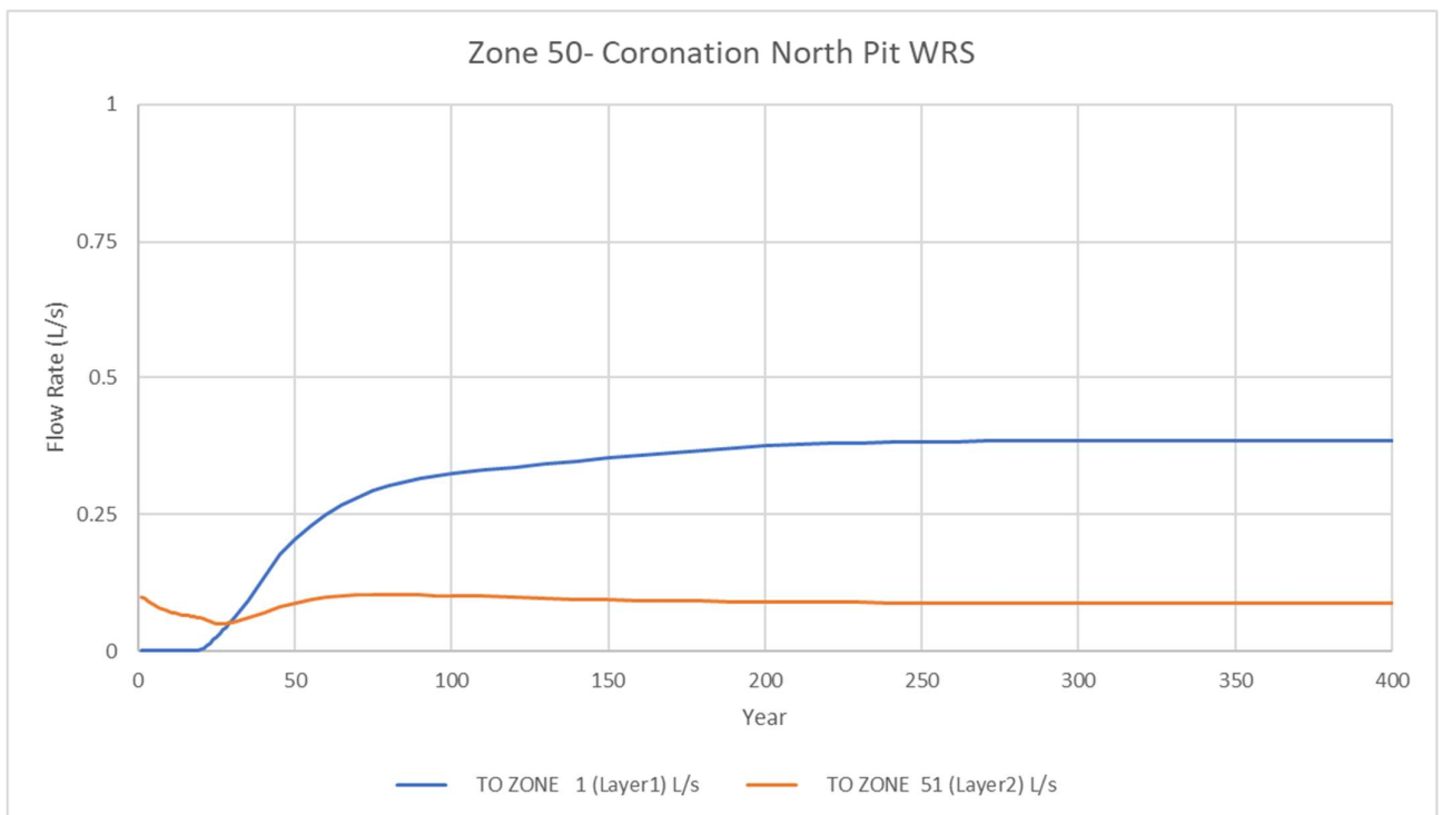
Figure 4.26 Seepage flow rate from Coronation North Pit WRS (zone 50) to Zone 1 (Layer 1) and Zone 51 (Layer 2)
