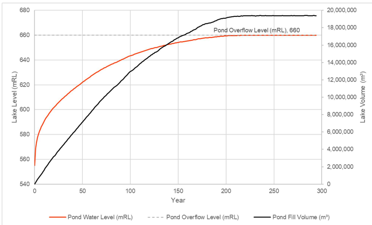
Figure 5.7 Coronation Pit Lake (CO6) filling assessment
