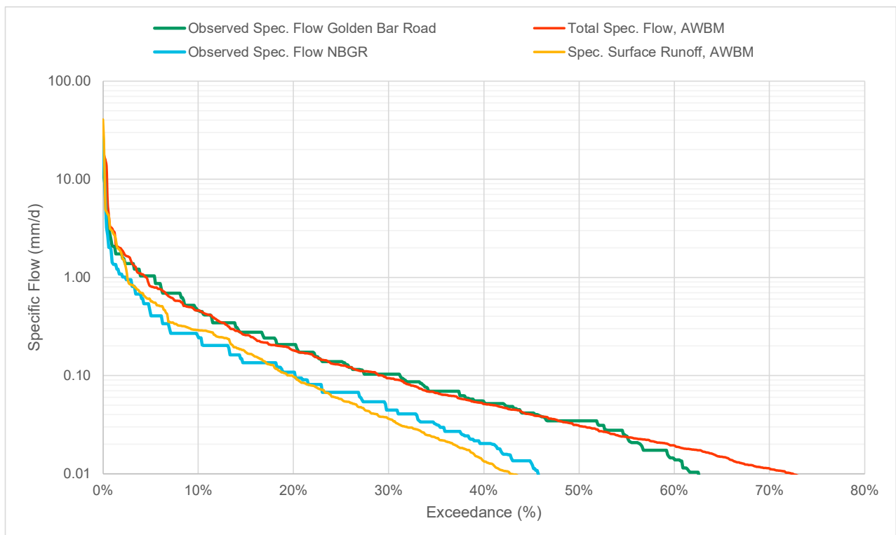
Figure 7.1 Calibration of the North Branch Waikouaiti River AWBM
