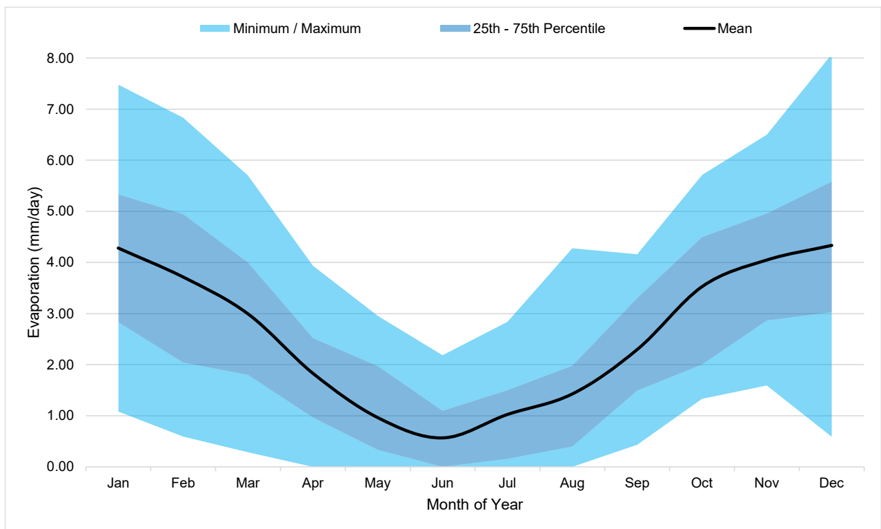
Figure 5.2 Evaporation statistics applied in WBM
