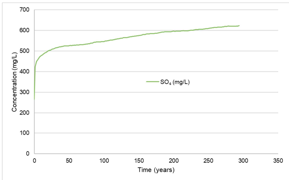
Figure 5.4 Coronation pit lake sulphate concentration (MWM, 2023)
