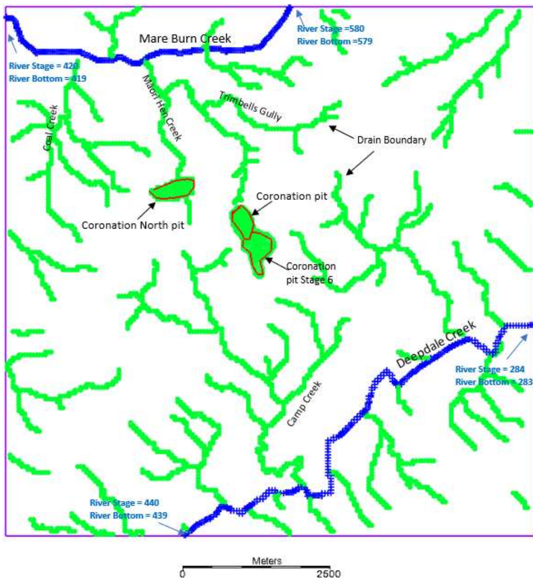
Figure 4.5 Coronation model surface boundary conditions.
