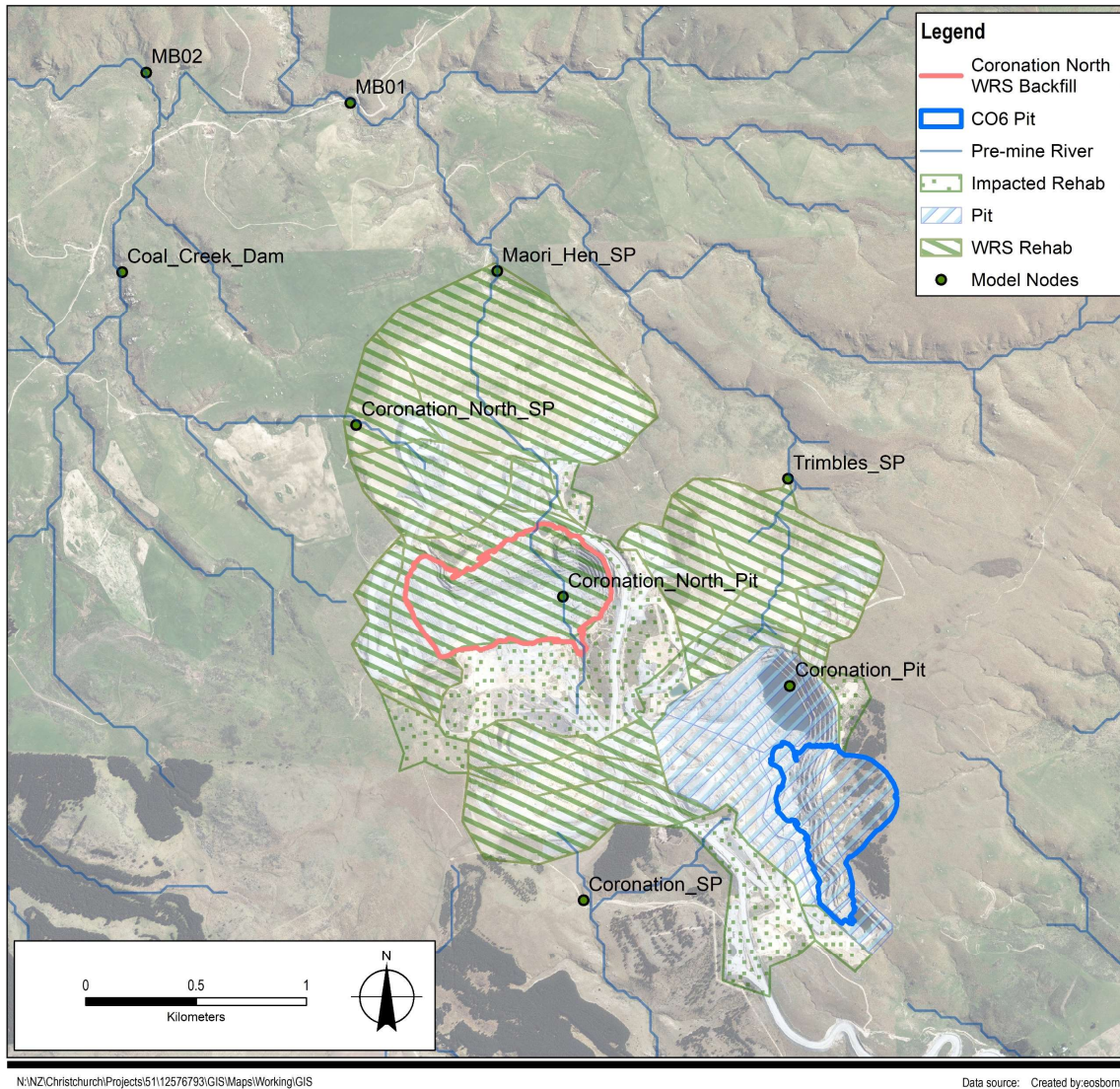
Figure 5.5 Coronation and Coronation North model domain
