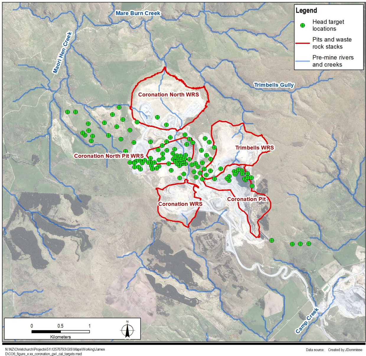
Figure 4.7 Groundwater head targets used in steady-state calibration
