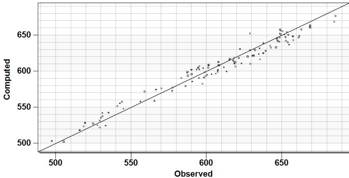
Figure 4.10 Steady state scatter plot (model computed vs observed head) using Table 4.2 hydraulic parameters
