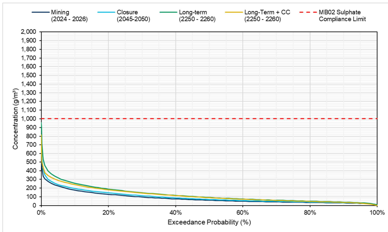
Figure 5.10 MB02 Sulphate – Modelled probability exceedance
