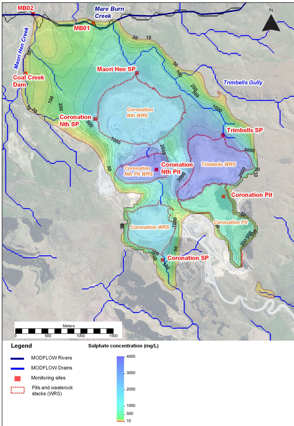
Figure 4.19 Contour plot showing plume extent after 400 years in model layer 1
