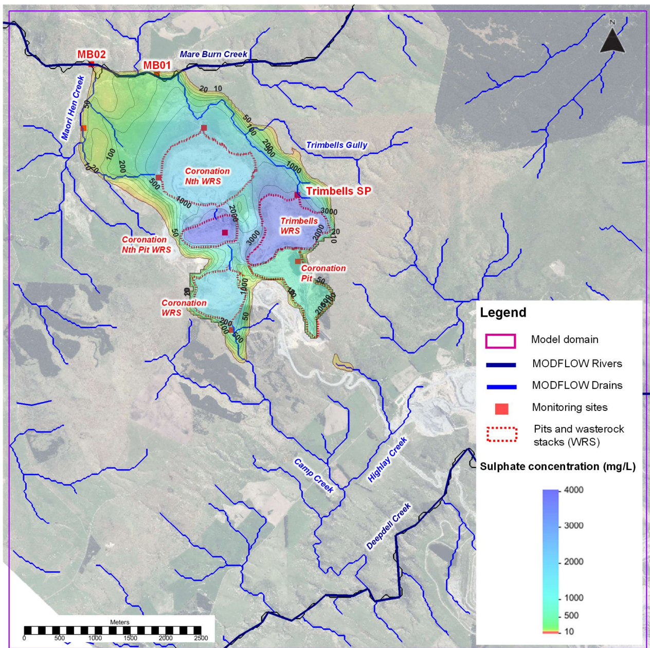
Figure 4.18 Contour plot showing plume after 400 years in model layer 1 within the entire model domain
