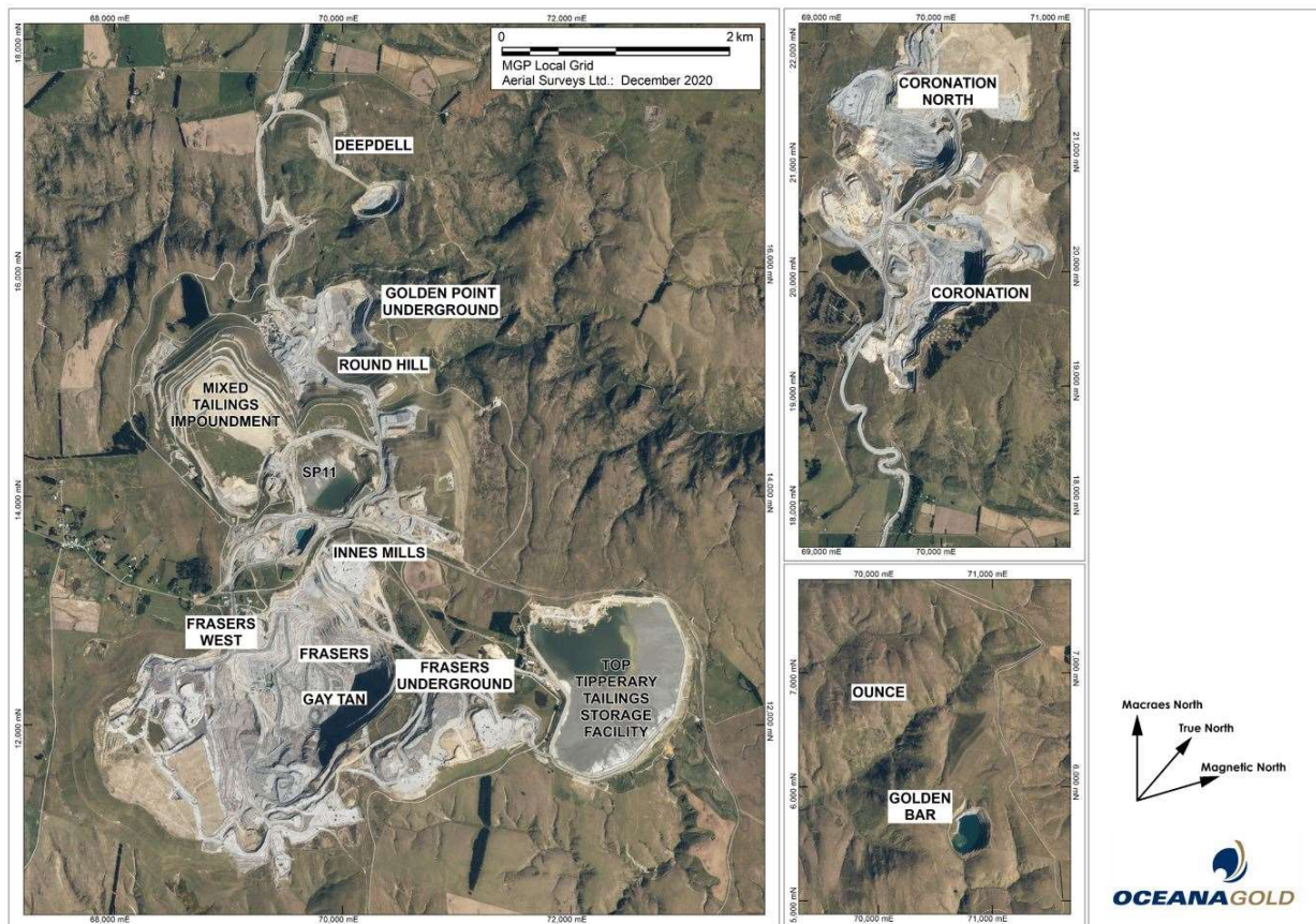
Figure 1.1 Macraes site plan
