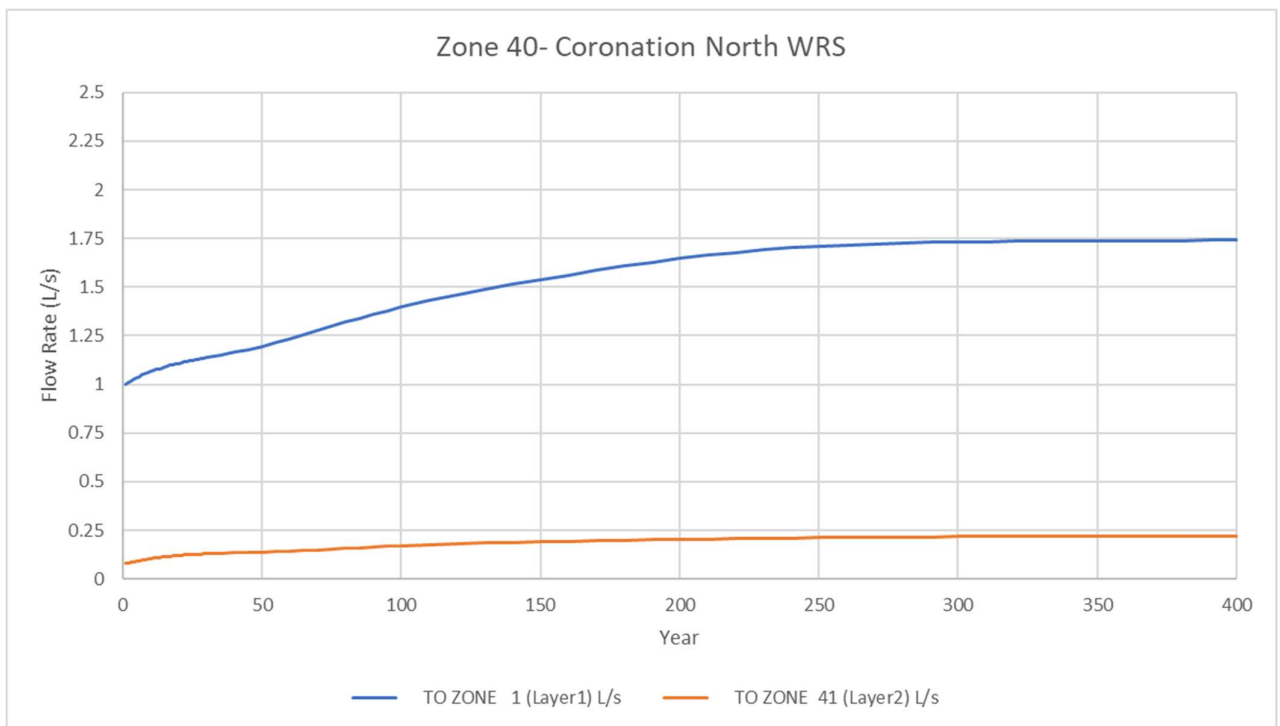
Figure 4.25 Seepage flow rate from Coronation North WRS (zone 40) to Zone 1 (Layer 1) and Zone 41 (Layer 2)
