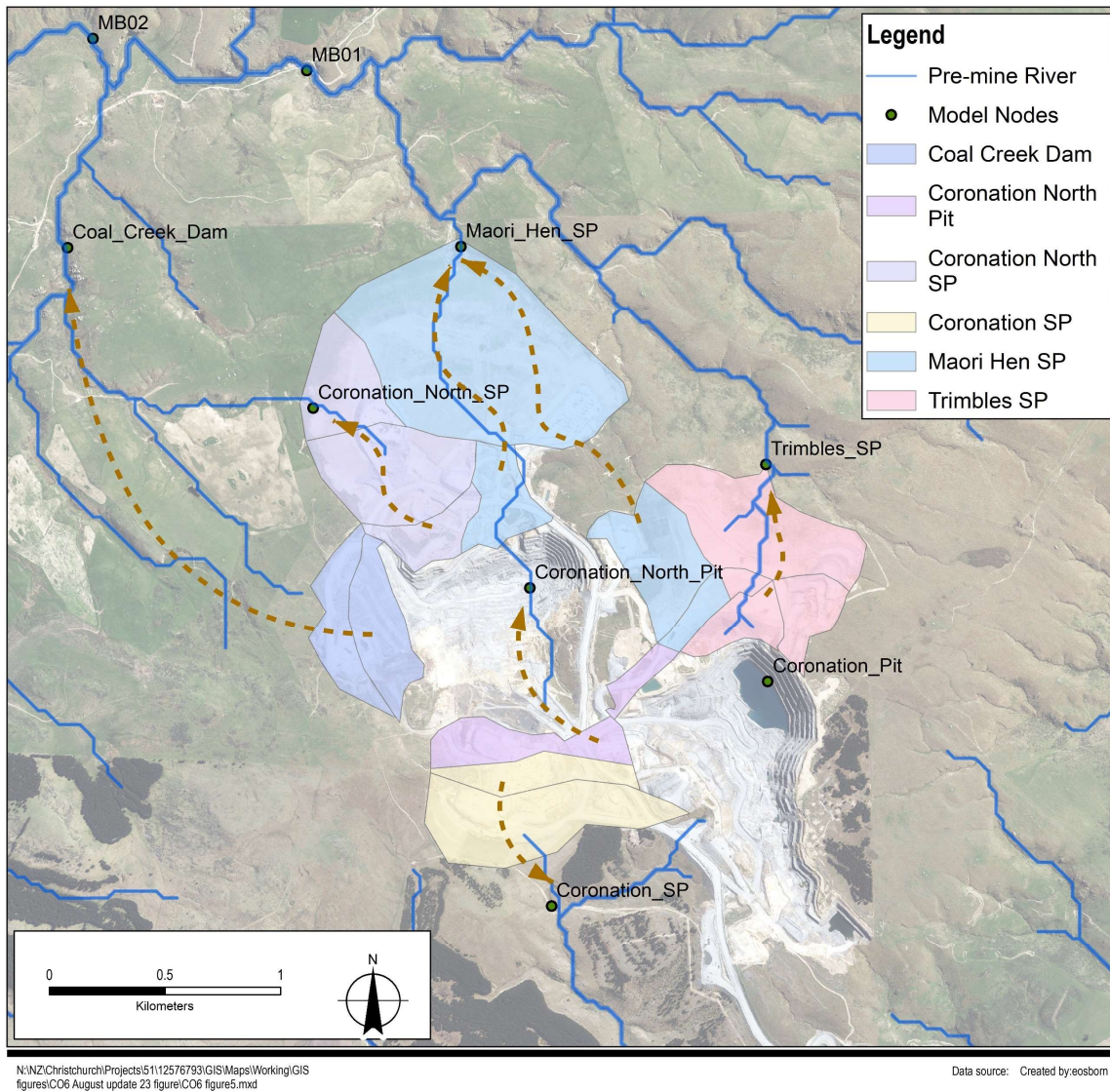
Figure 7.6 Coronation Seepage Catchment Map - Current
