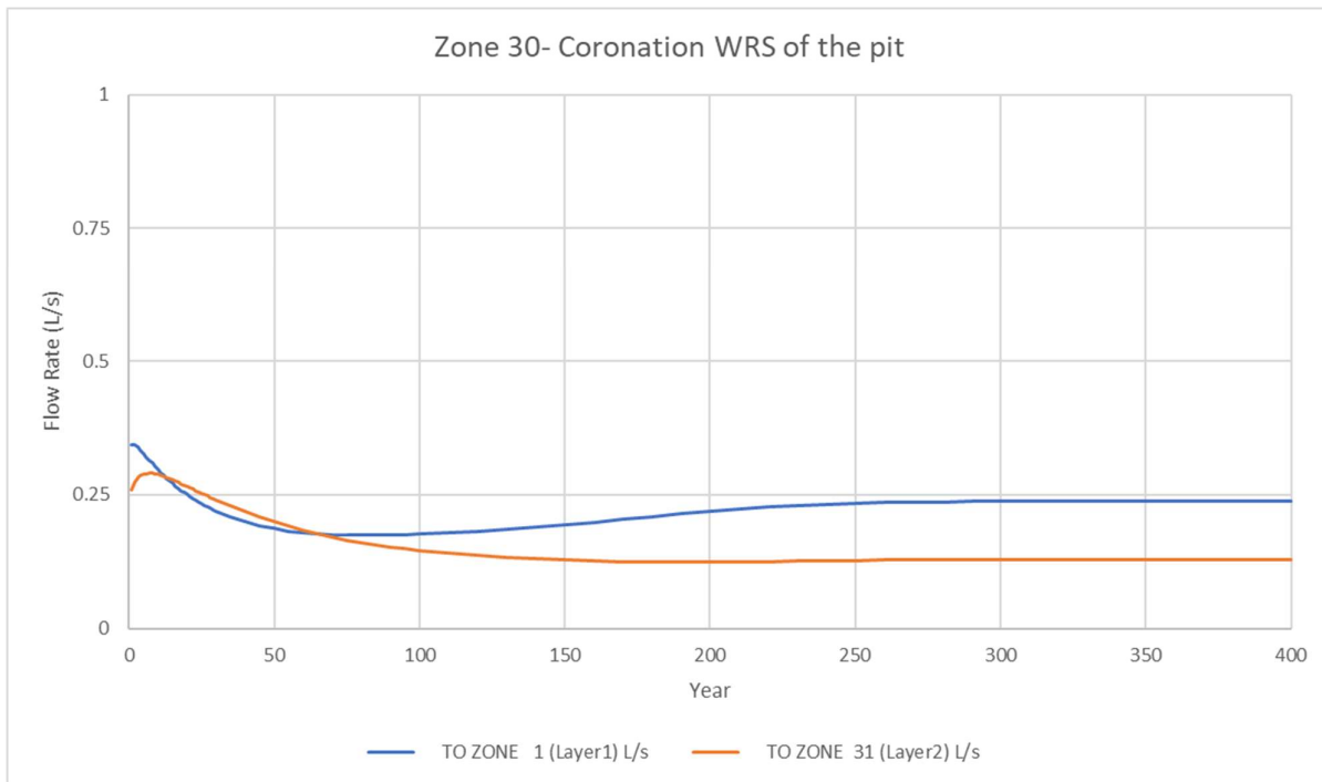
Figure 4.24 Seepage flow rate from Coronation WRS (zone 30) to Zone 1 (Layer 1) and Zone 31 (Layer 2)
