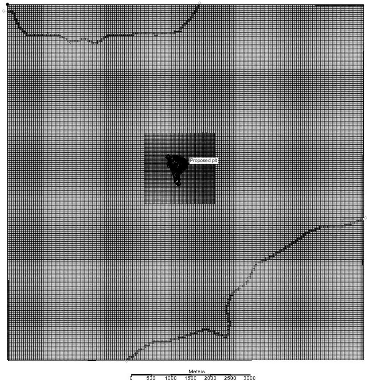
Figure 4.4 Coronation model grid design
