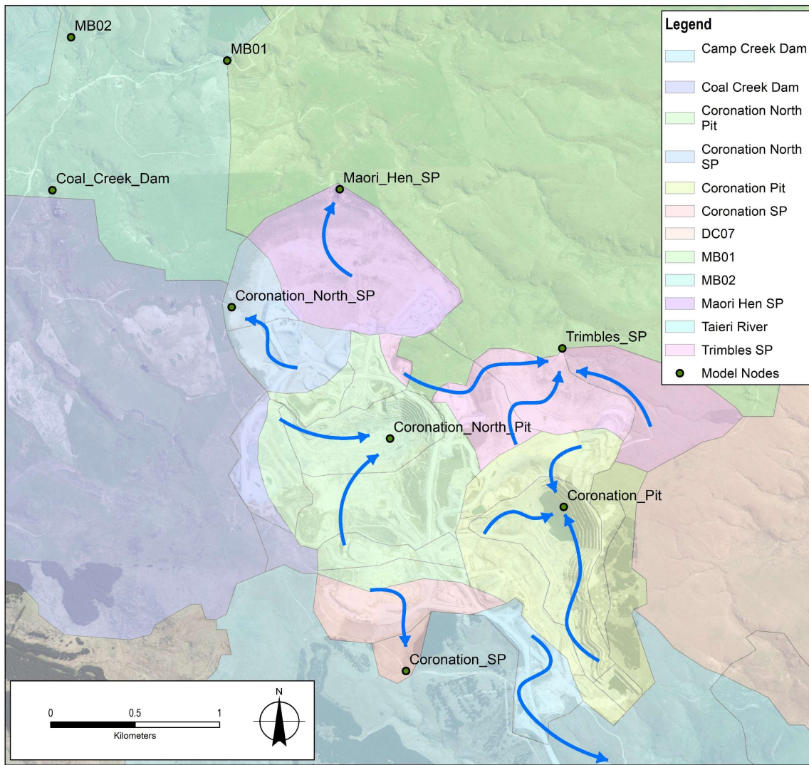
Figure 7.4 Coronation Catchment Map - Current
