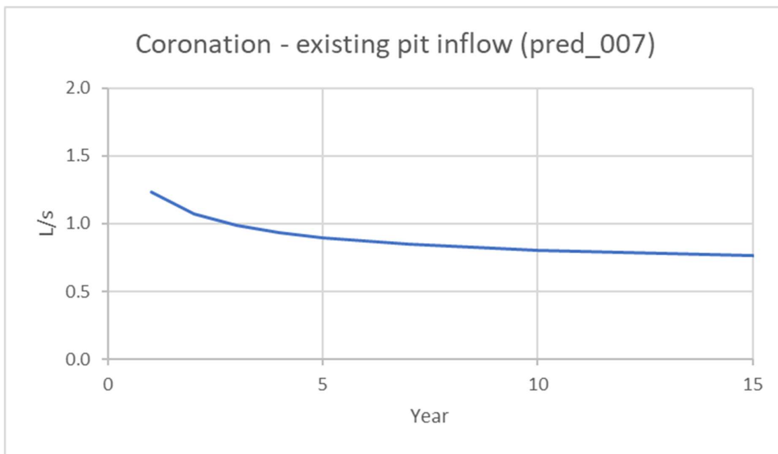
Figure 4.13 Existing pit inflow (Coronation pit)
