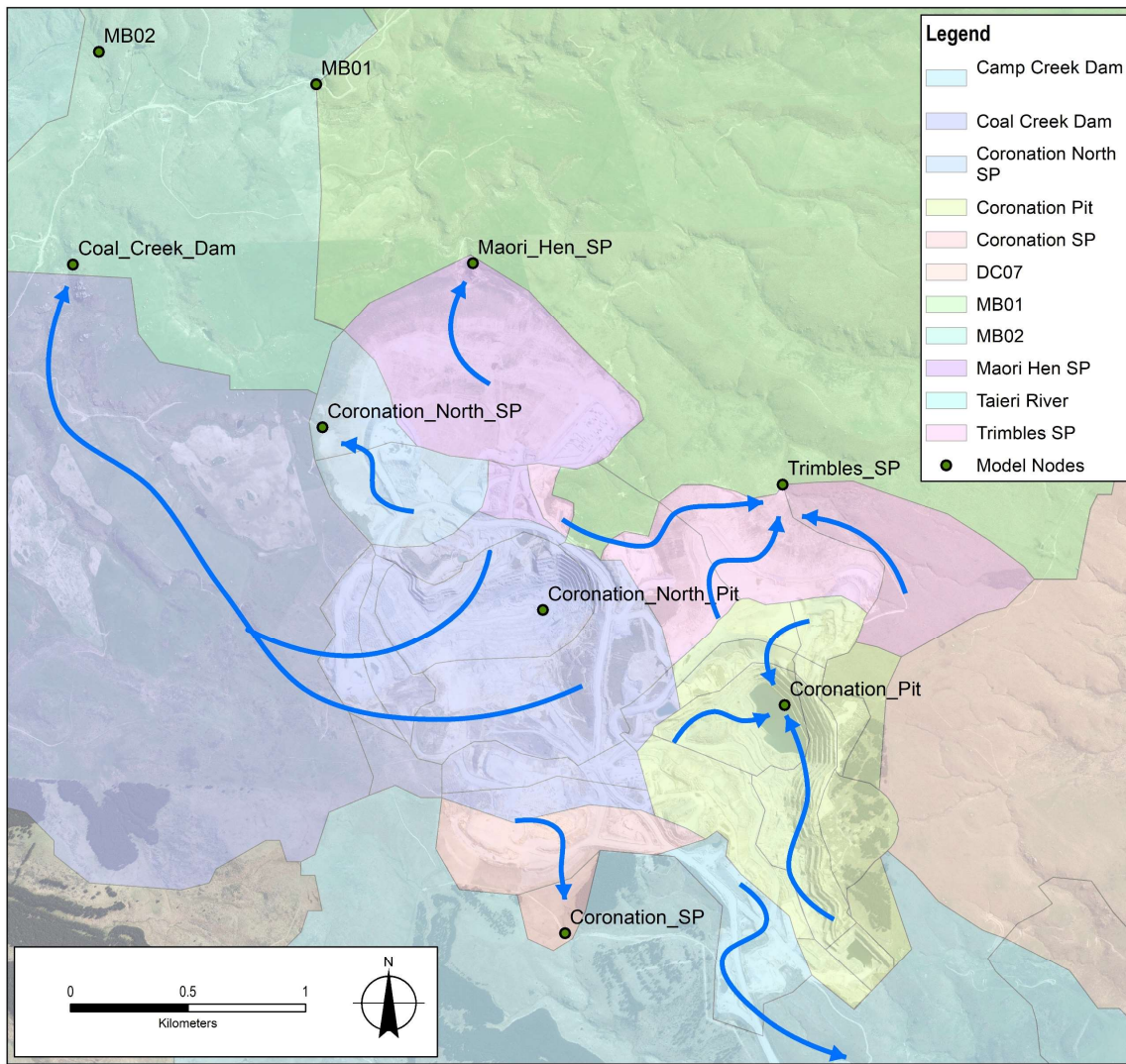
Figure 7.5 Coronation Catchment Map - Closure
