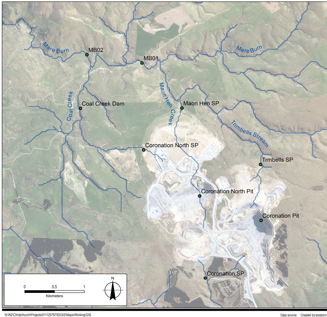
Figure 3.3 Key surface water features relating to the Coronation Stage 6 expansion
