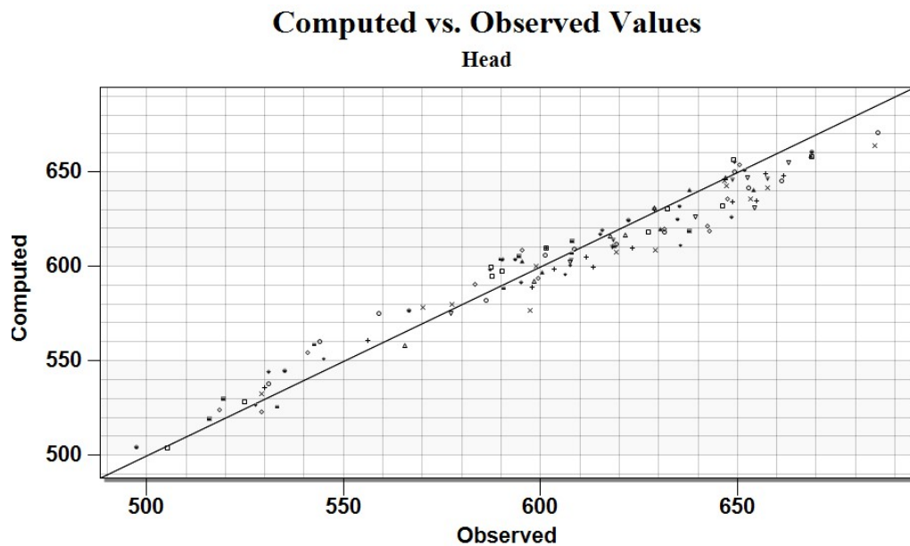
Figure 4.8 Steady state scatter plot (model computed vs observed head)
