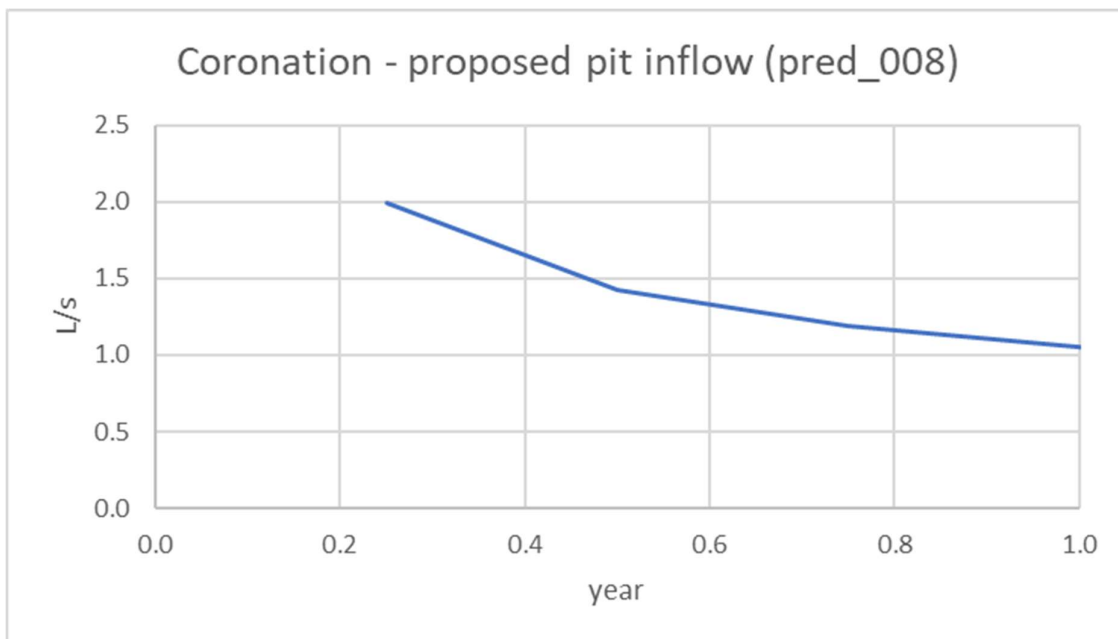
Figure 4.14 Proposed pit inflow (Coronation pit)
