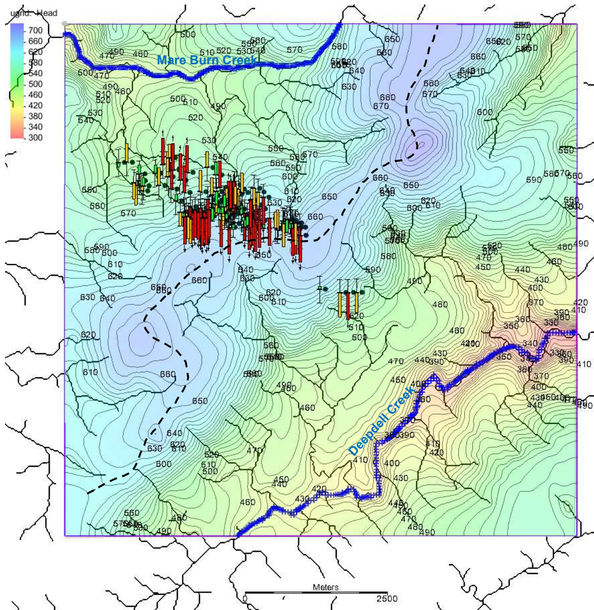
Figure 4.11 Steady-state modelled head contours (pre mining))
