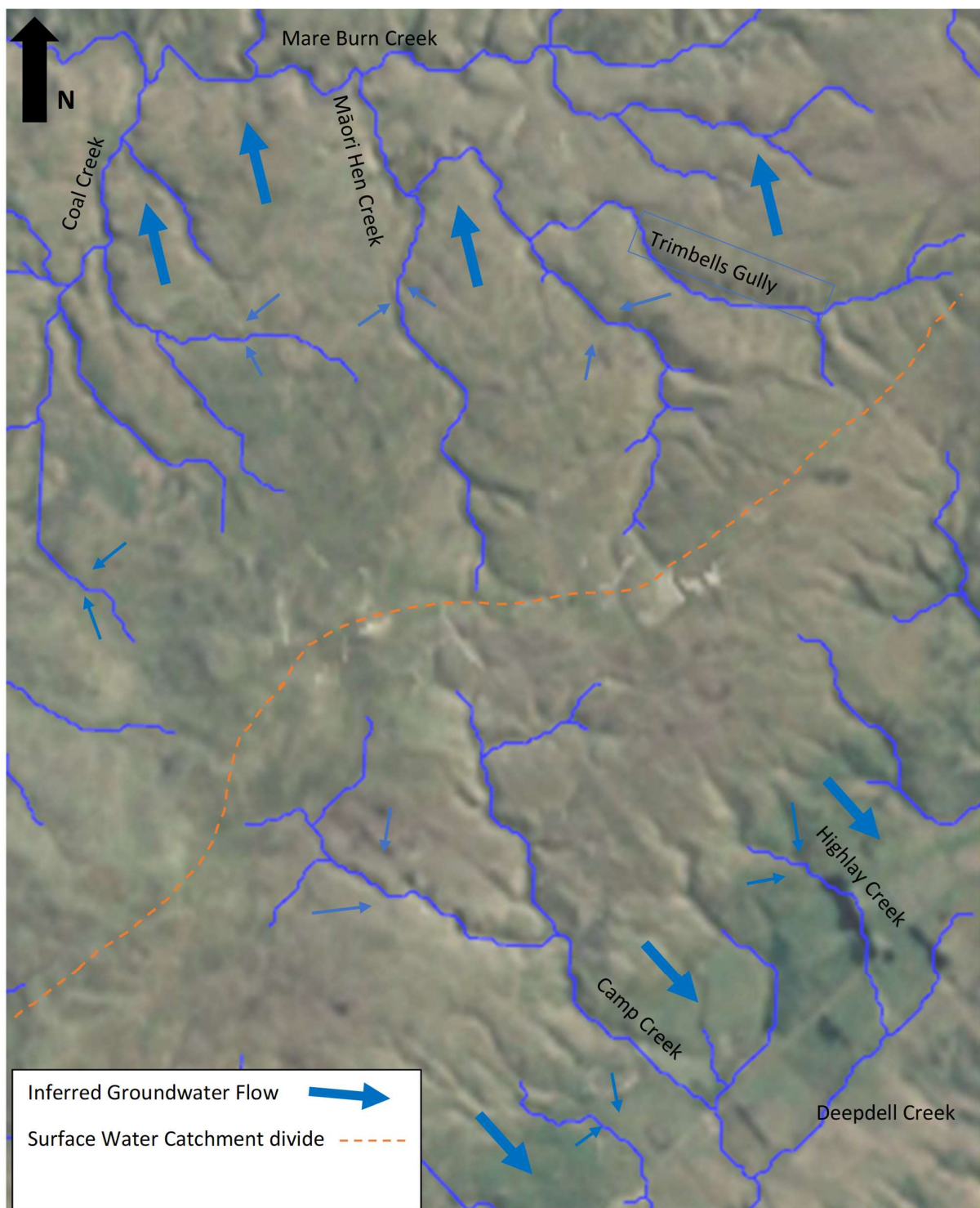
Figure 4.1 Inferred groundwater flow direction pre mining
