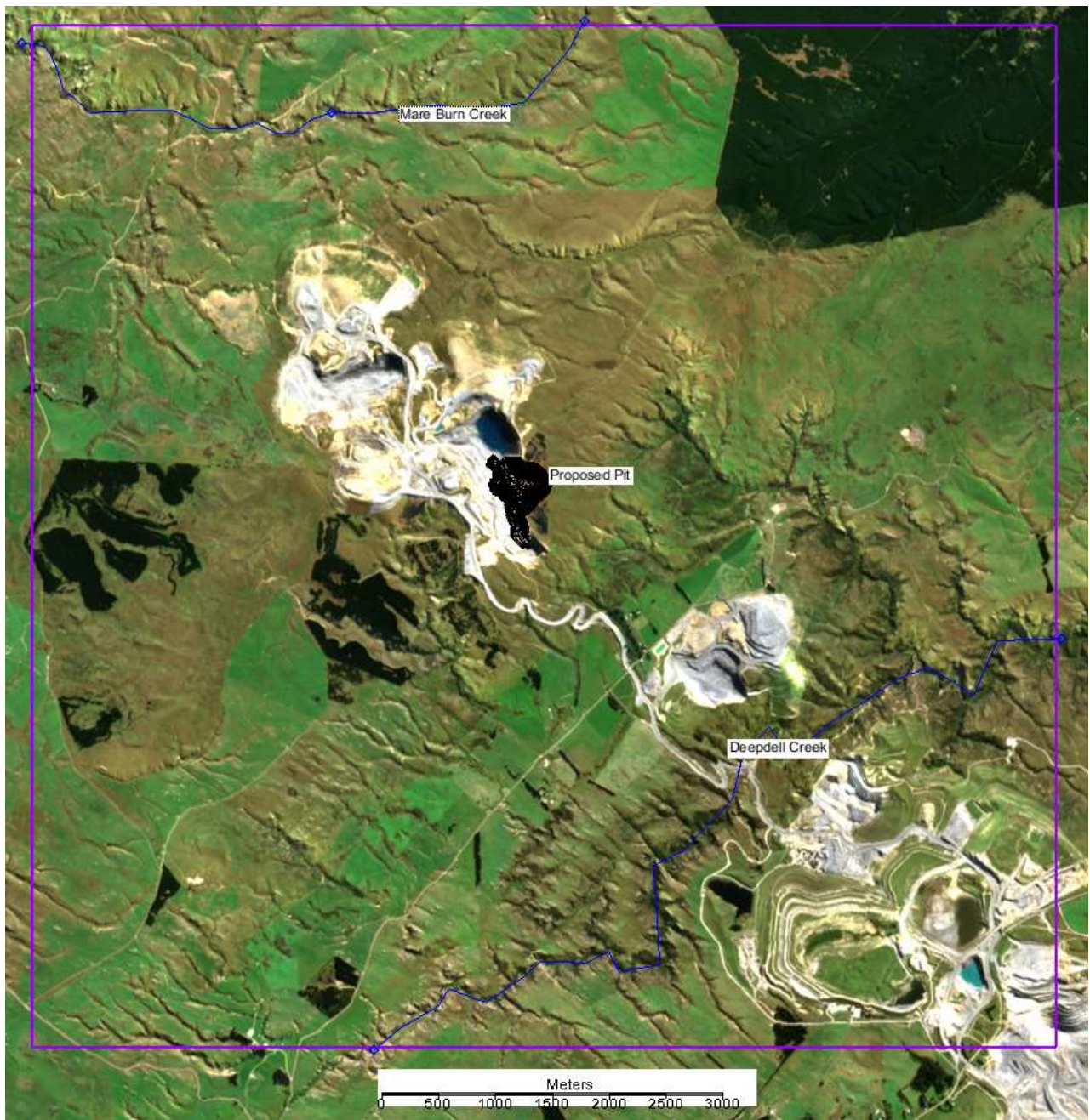
Figure 4.3 Coronation model domain
