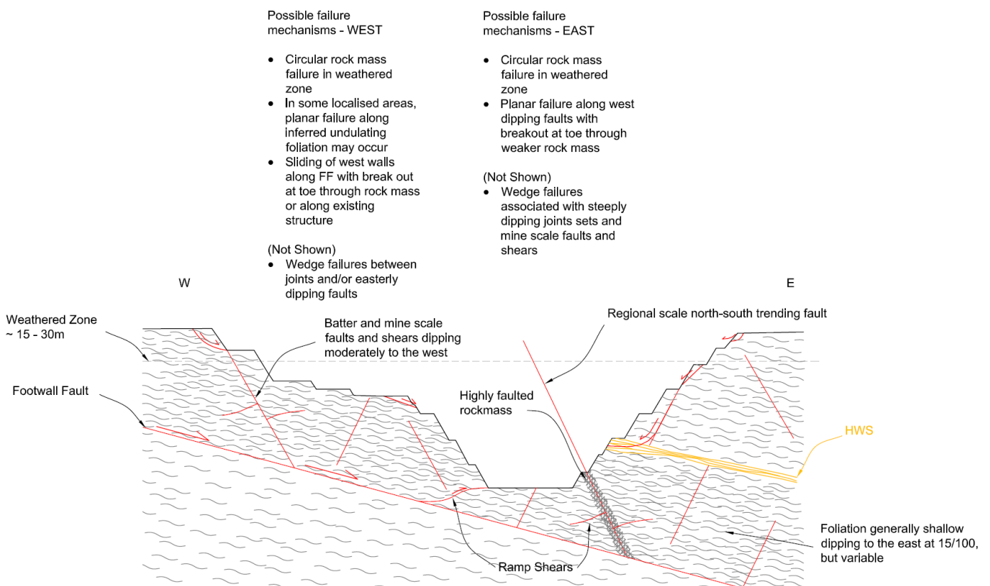
Inset 7: Schematic section of geotechnical model and failure mechanisms at Macraes.
