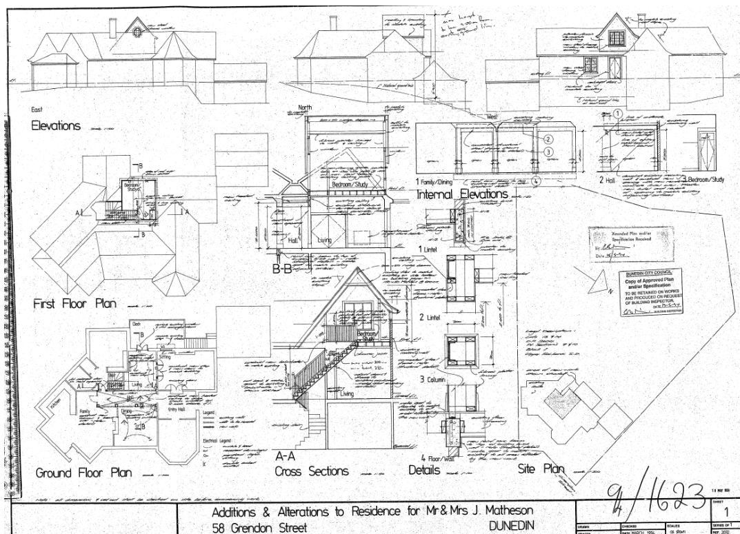
Plans dated 1994 showing the bedroom/study space additions extending through the original roof. Source DCC Property File
