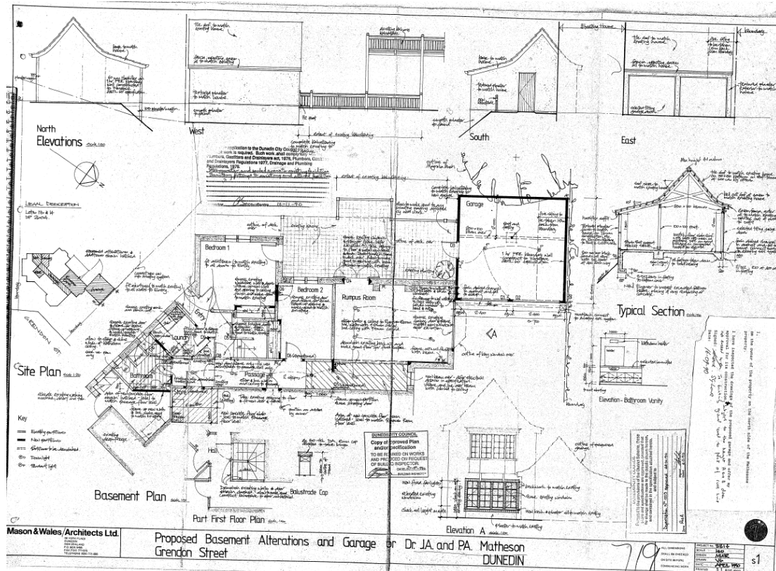
Plans dated 1990 showing the proposed single storey garage constructed in roughly the same location as shown on the original plans. Source DCC Property File
