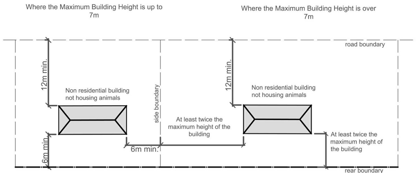
Figure 17.6.9.1C: Setbacks for non-residential buildings that do not house animals
