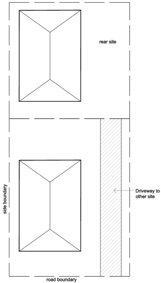
Figure 15.6.10A: Site coverage calculation
