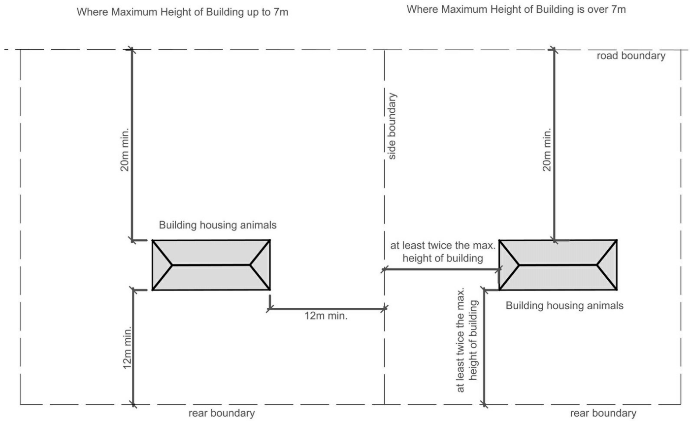
Figure 16.6.10.1B: Setbacks for non-residential buildings that house animals
