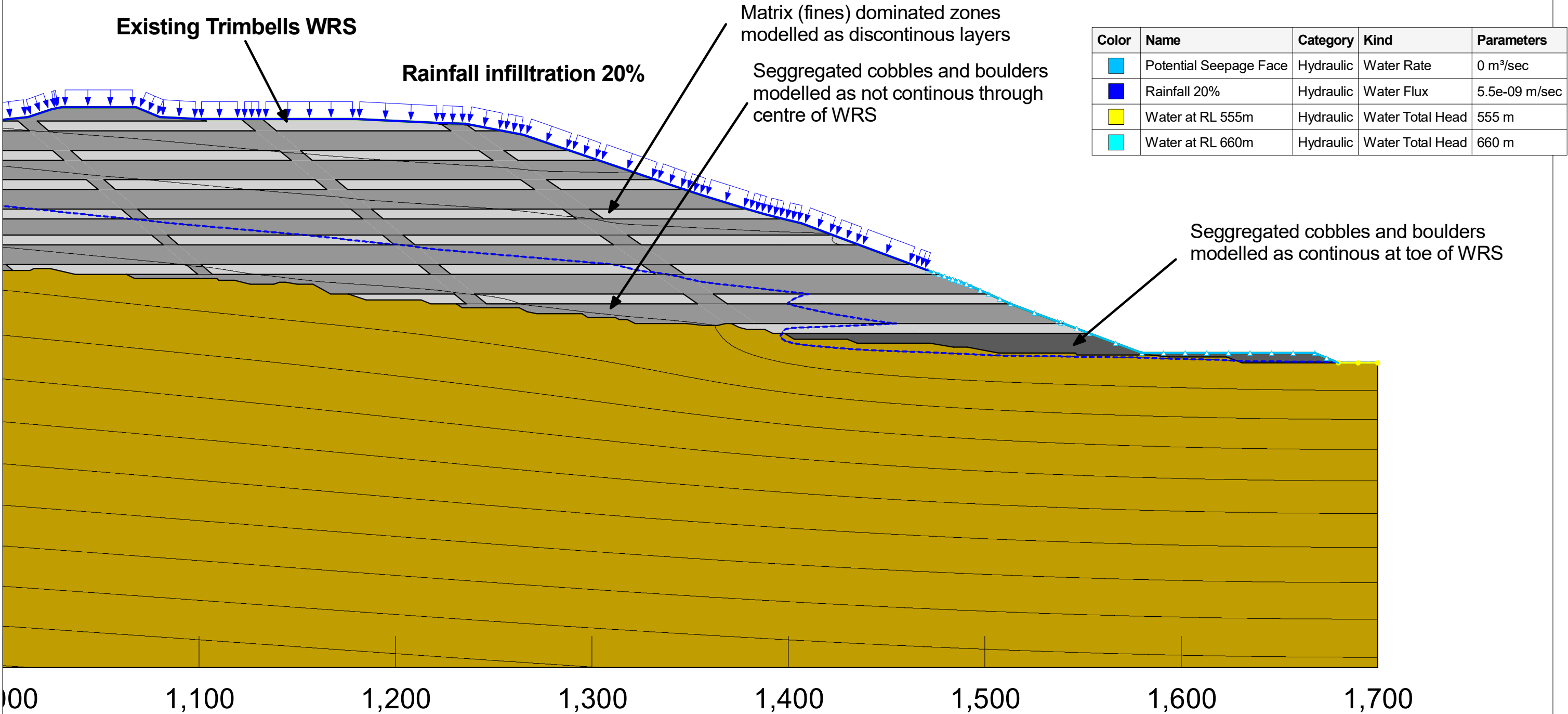
Seepage analysis for pore pressure profile
