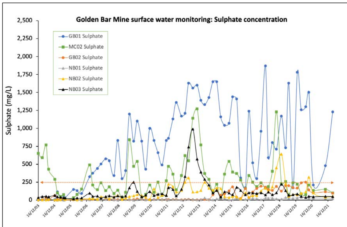
Figure 4. Sulphate concentrations over time at surface water monitoring sites in the vicinity of the Golden Bar Mine. Dashed horizontal line indicates the consent compliance limit for Waikouaiti River North Branch monitoring and compliance site NB03.
