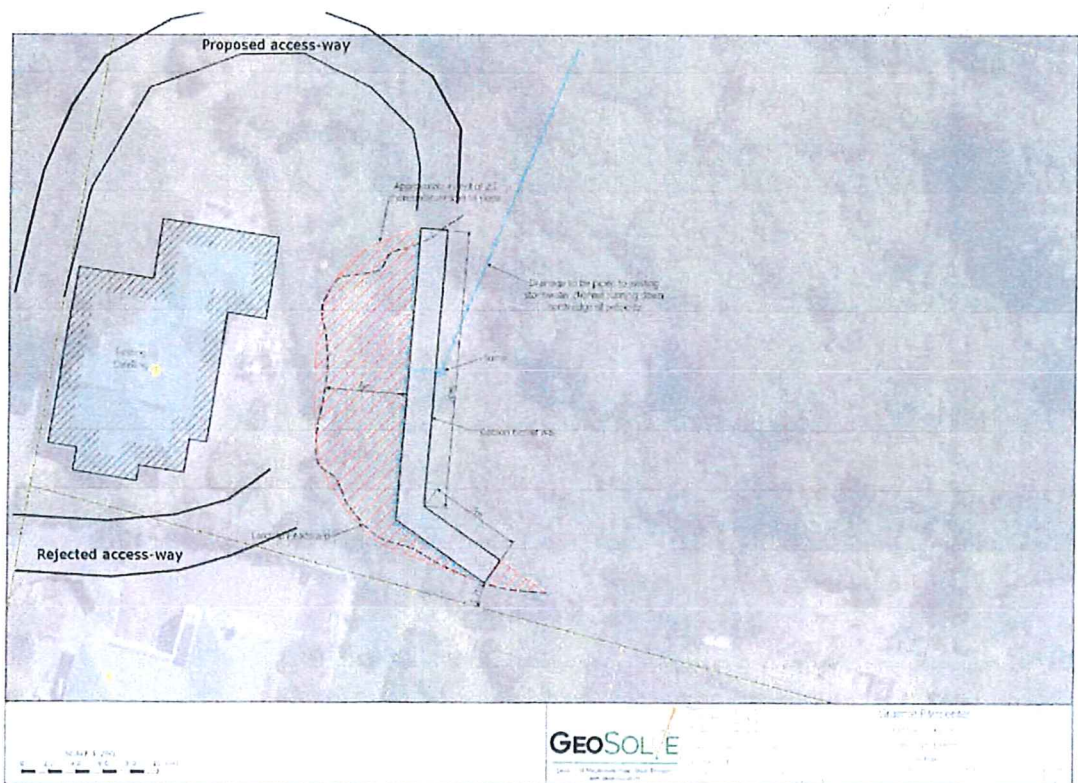
Photo 14. Proposed vehicle access-way to the slip area showing also the rejected alternative.
