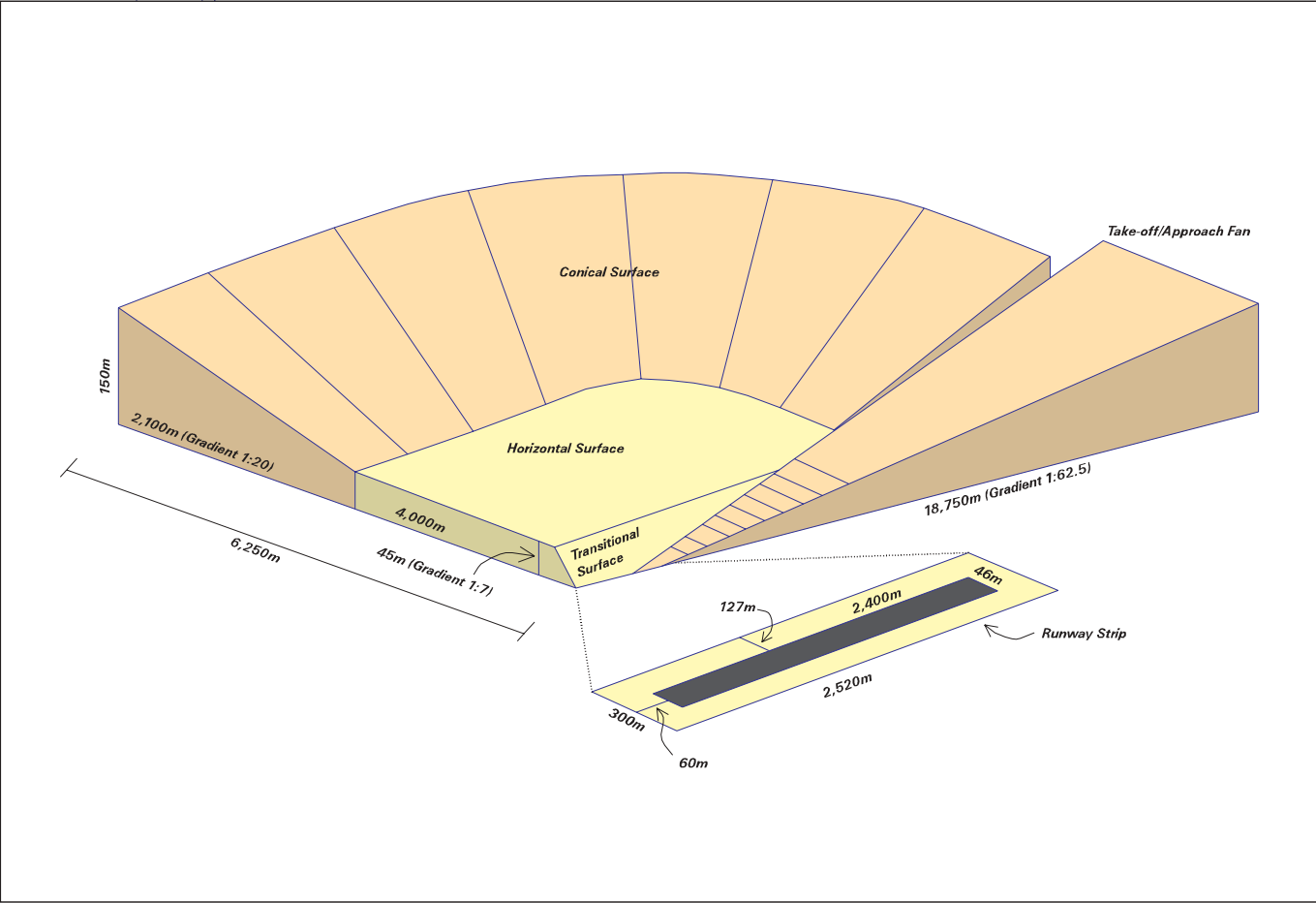
Obstacle Limitation Surface
