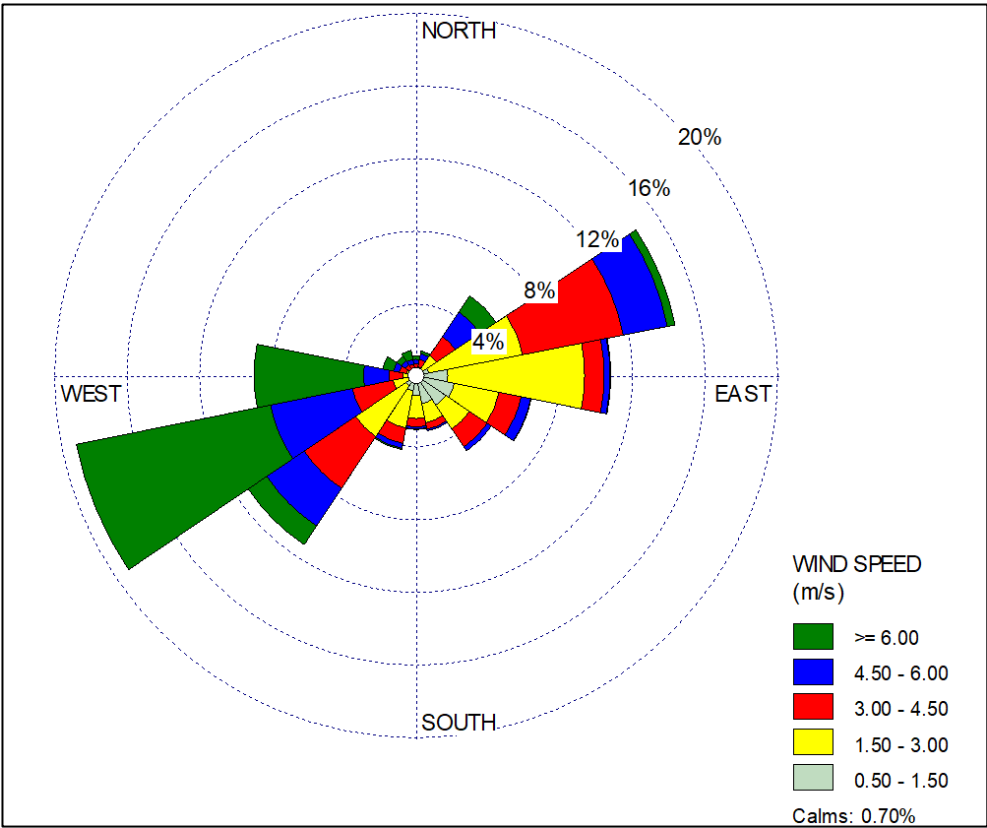
Figure 8-3: TAPM output wind rose - Dunedin Airport AWS location (2017-2019) – average wind speed = 4.0 m/s
