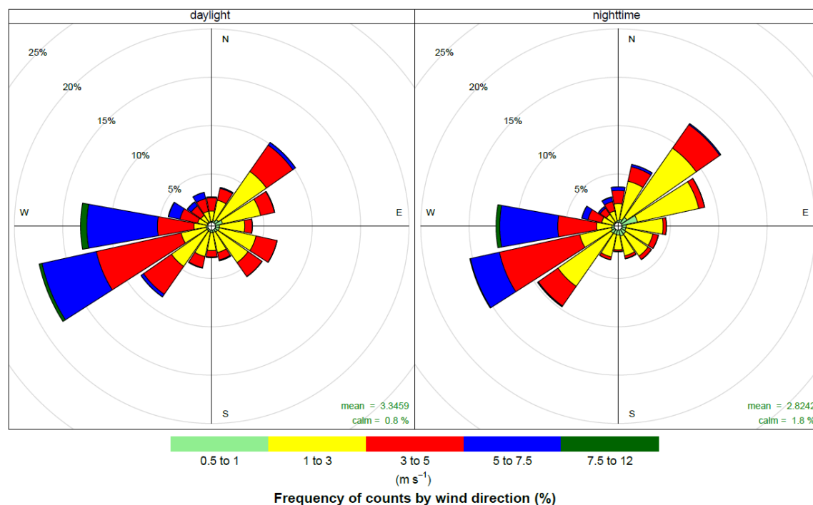
Figure 9-2: Wind rose of daytime/night-time hours
