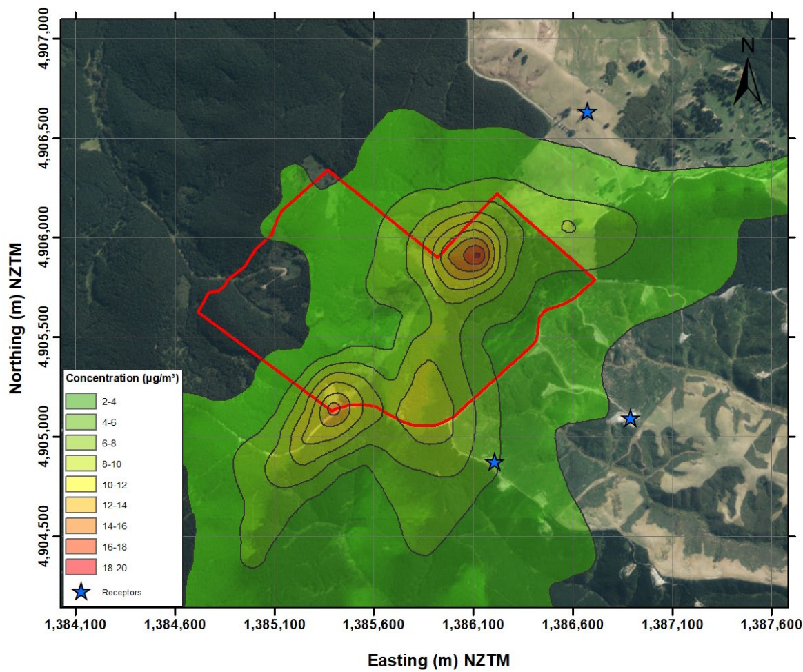
Figure 11-2: Maximum predicted 1-hour SO 2 concentrations (µg/m 3 )
