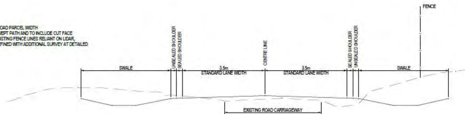
TYPICAL SECTION SCALE 1:50
