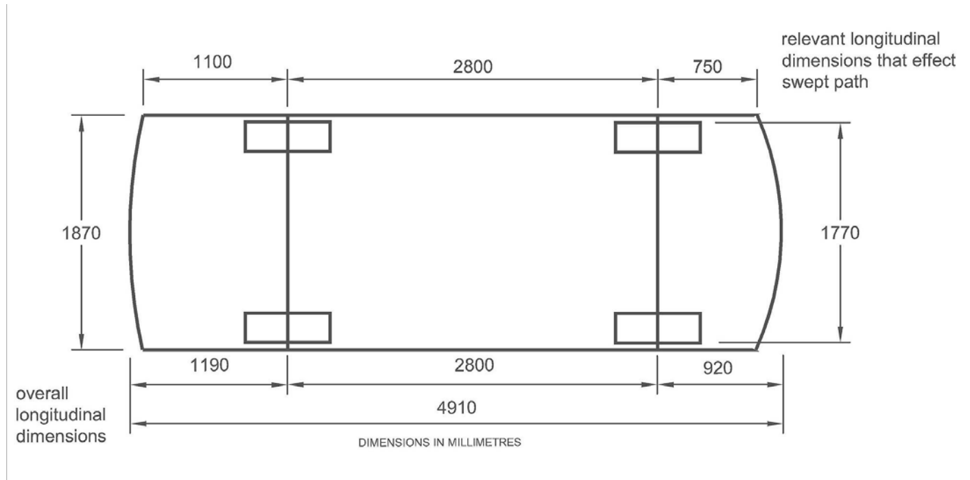
Figure 6B.8 85th percentile vehicle dimensions
