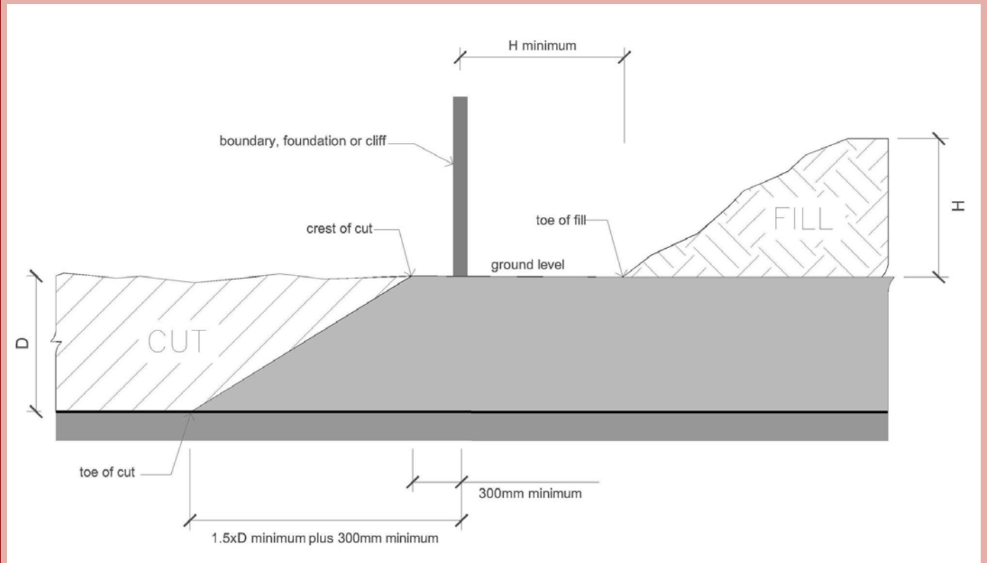
Figure 8A.5.4A: Unsupported cut and fill (elevation view)
