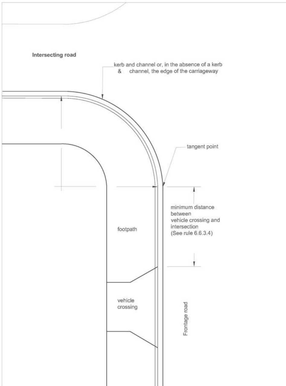
Figure 6B.17 Method to determine minimum sight distance between vehicle crossing and intersection
