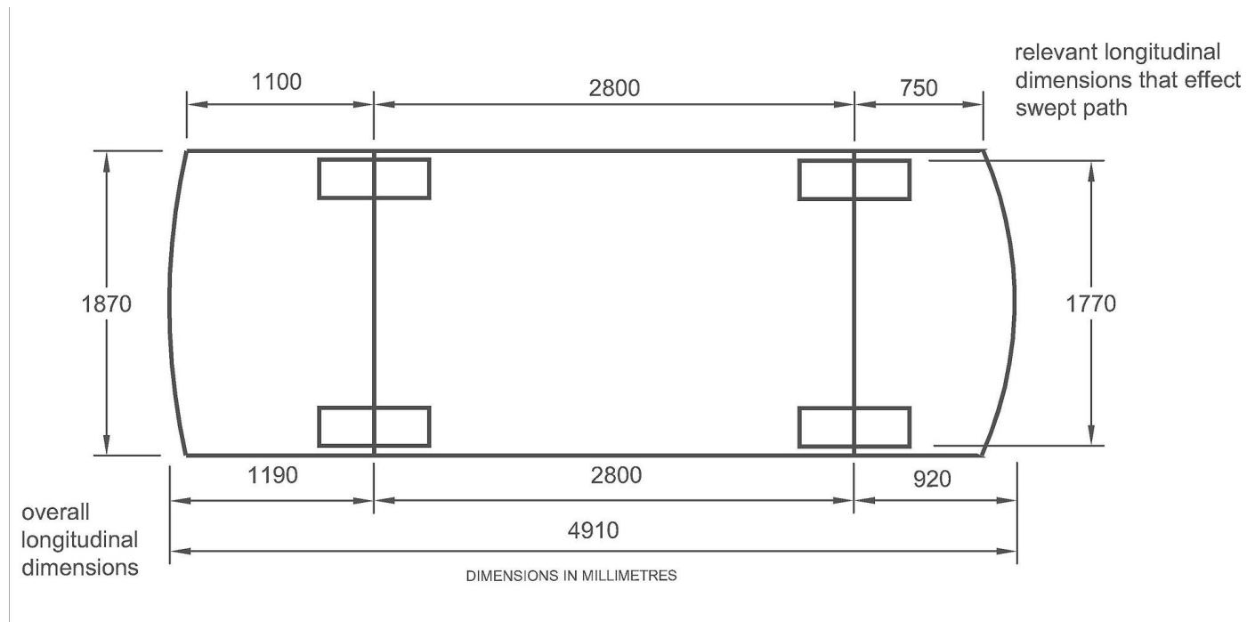
Figure 6B.8 85th percentile vehicle dimensions
