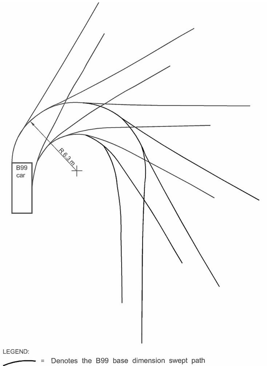
Figure 6B.7 99th percentile vehicle turning circle
