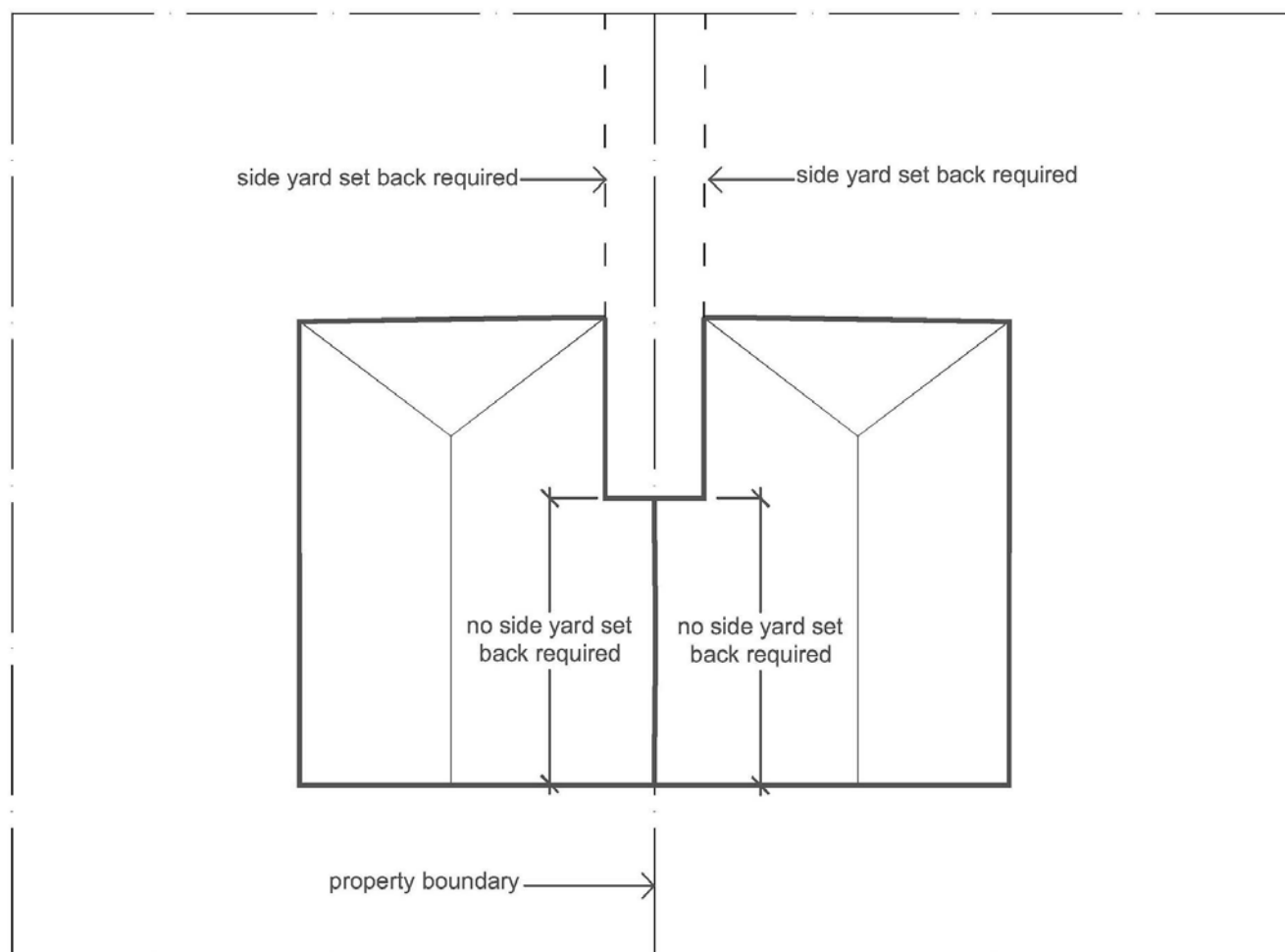
Figure 15.6.13.1B: Setbacks for buildings sharing common wall
