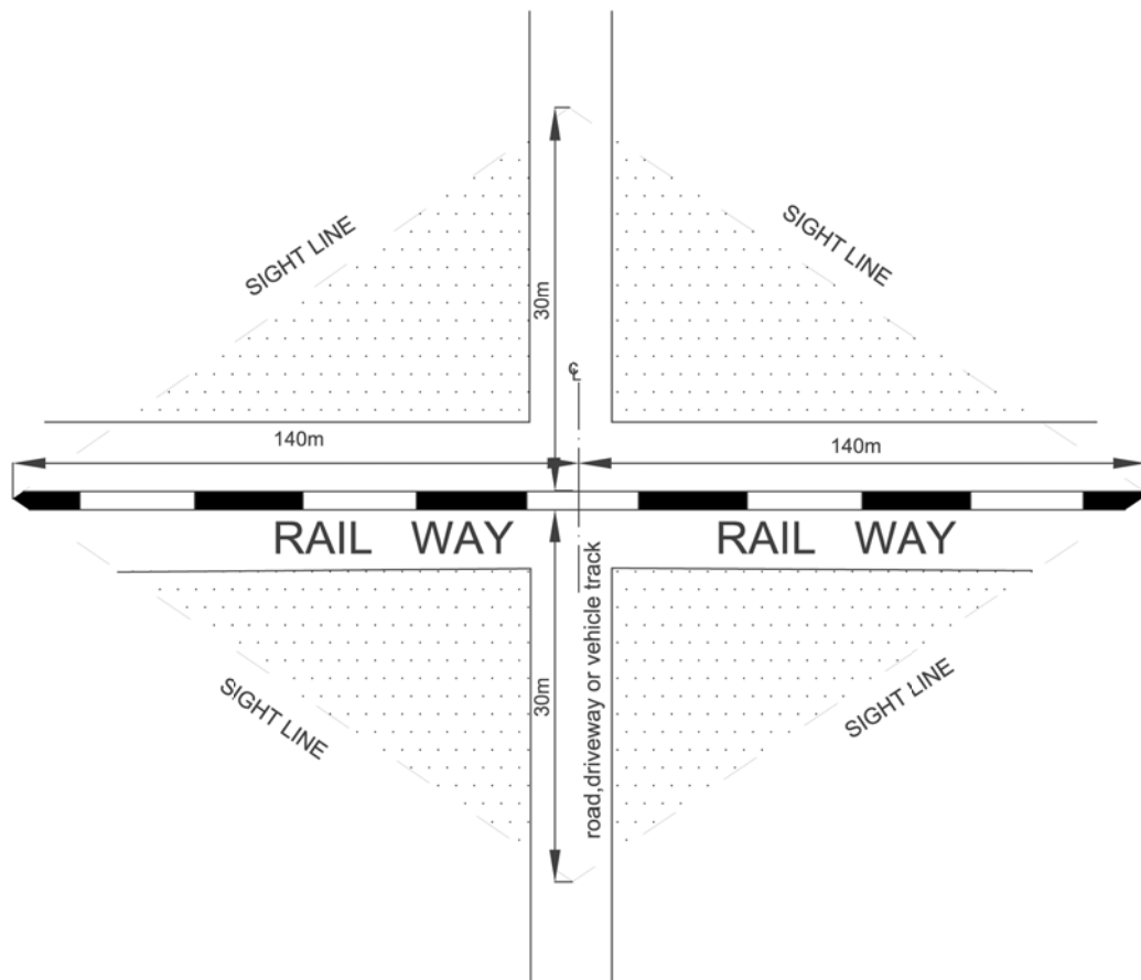
Figure 6B.18 Railway level crossing sight line restrictions
