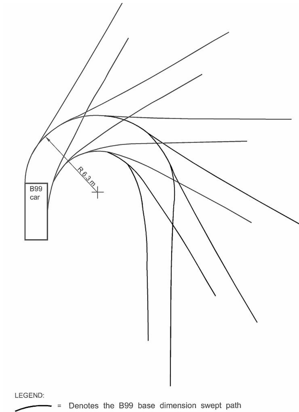
Figure 6B.7 99th percentile vehicle turning circle
