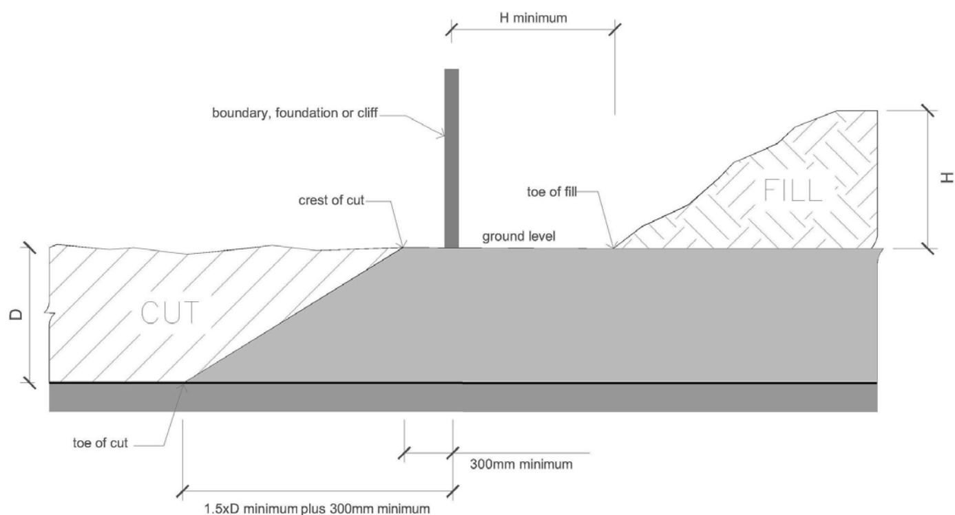
Figure 8A.5.4A: Unsupported cut and fill (elevation view)
