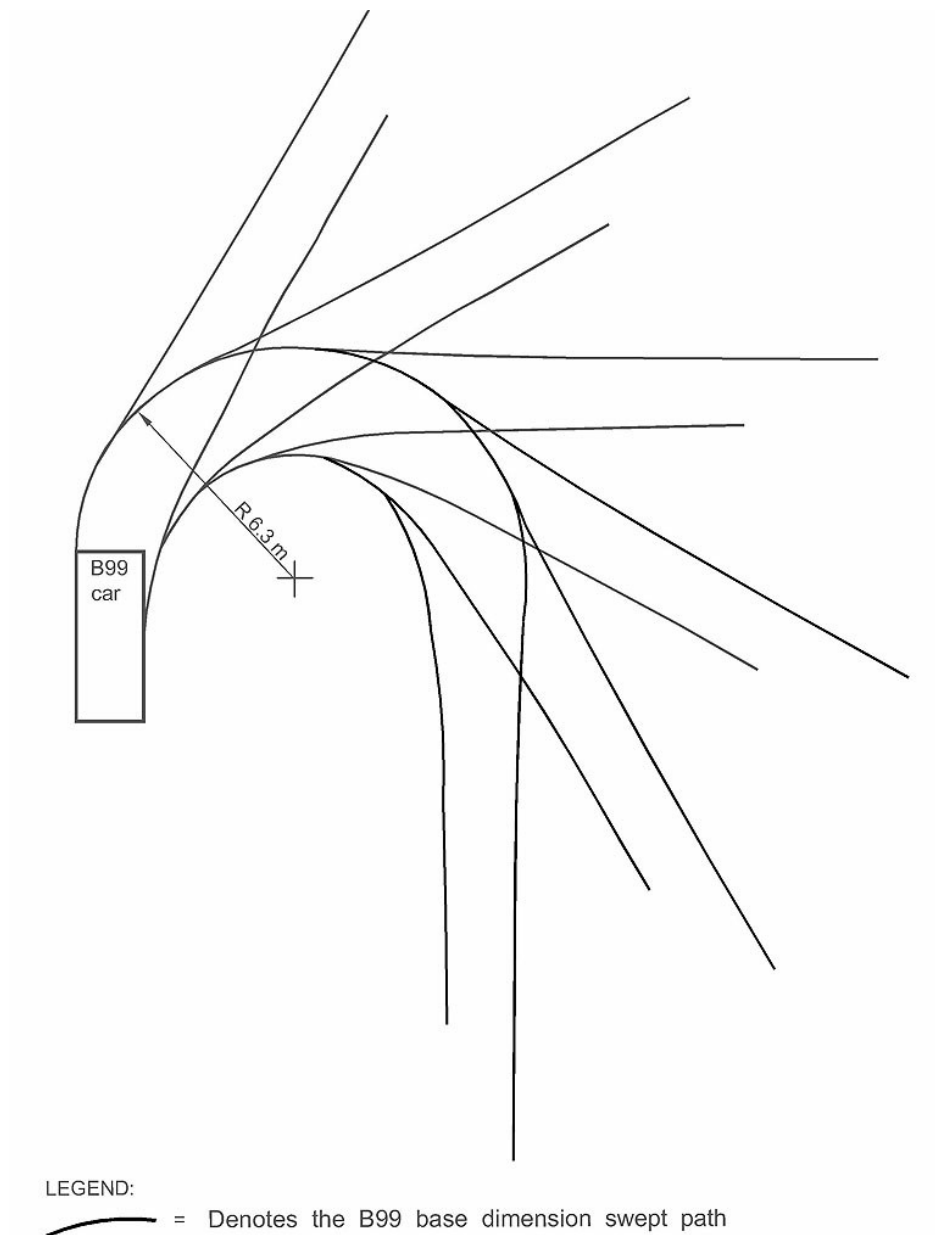
Figure 6B.7 99th percentile vehicle turning circle
