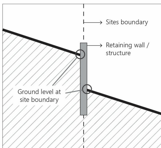
Figure 1.4.1AA: Ground level when a retaining wall/structure crosses a site boundary {Change D18}
