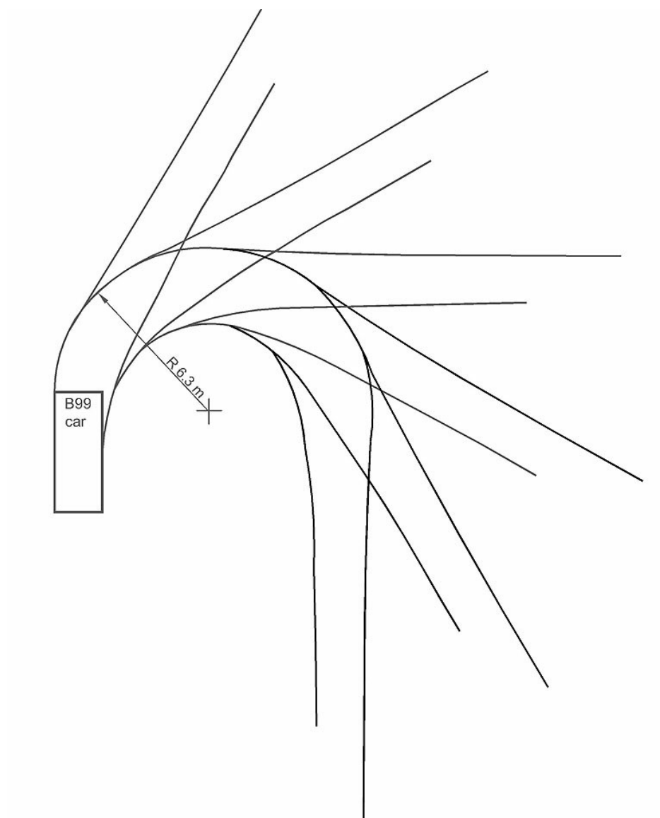
Figure 6B.7 99th percentile vehicle turning circle
