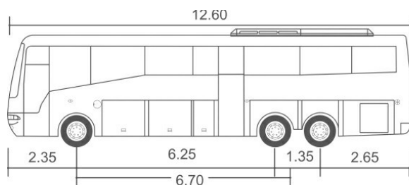
DESIGN VEHICLE DIMENSIONS (metres)
