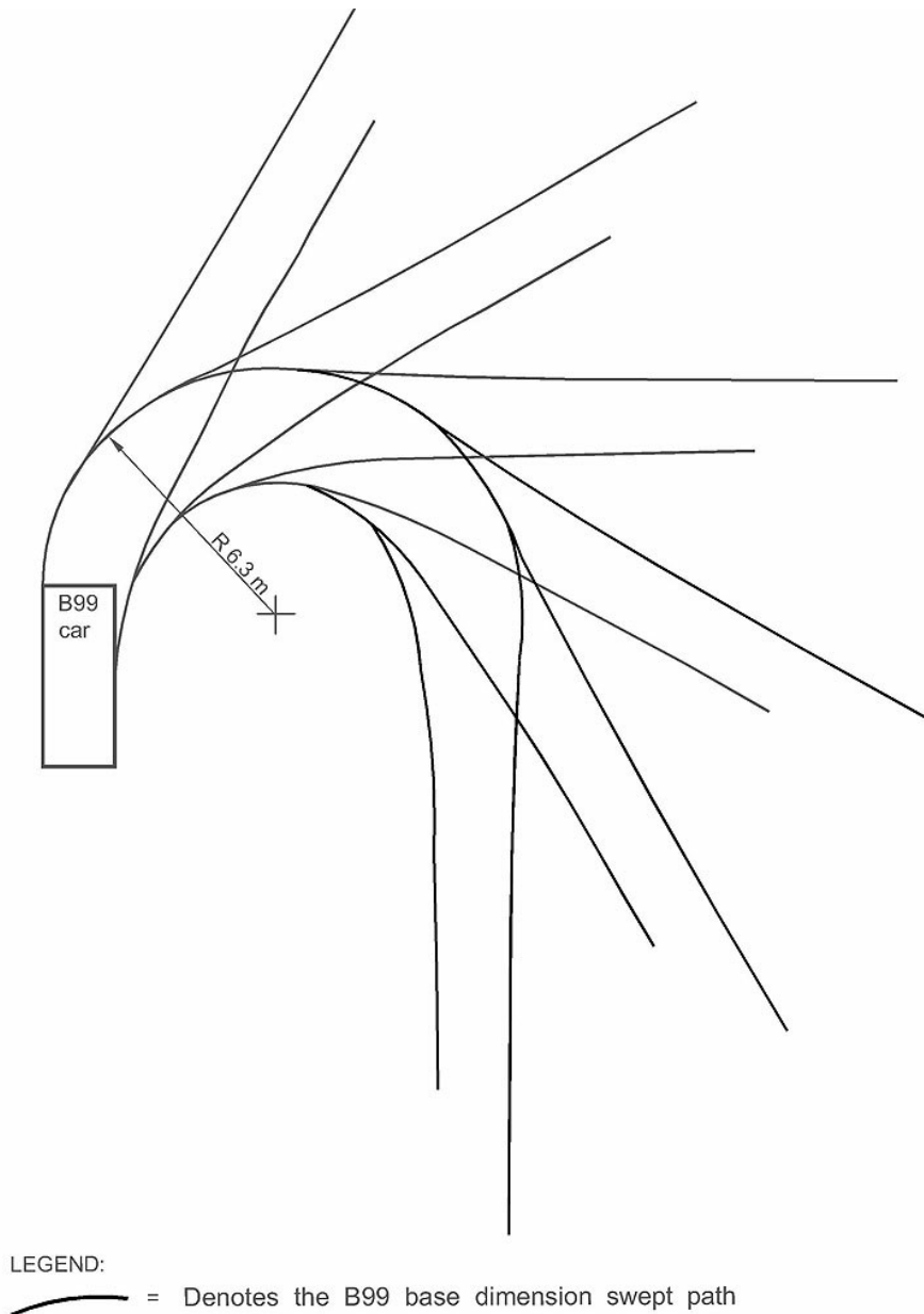
Figure 6B.7 99th percentile vehicle turning circle
