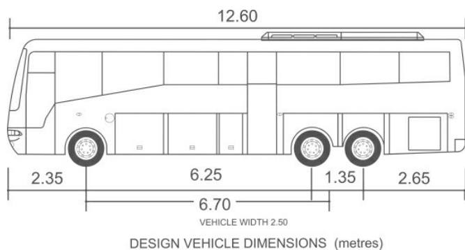
Figure 6B.12 Coach turning circle
