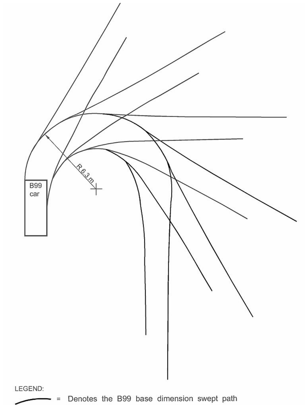
Figure 6B.7 99th percentile vehicle turning circle
