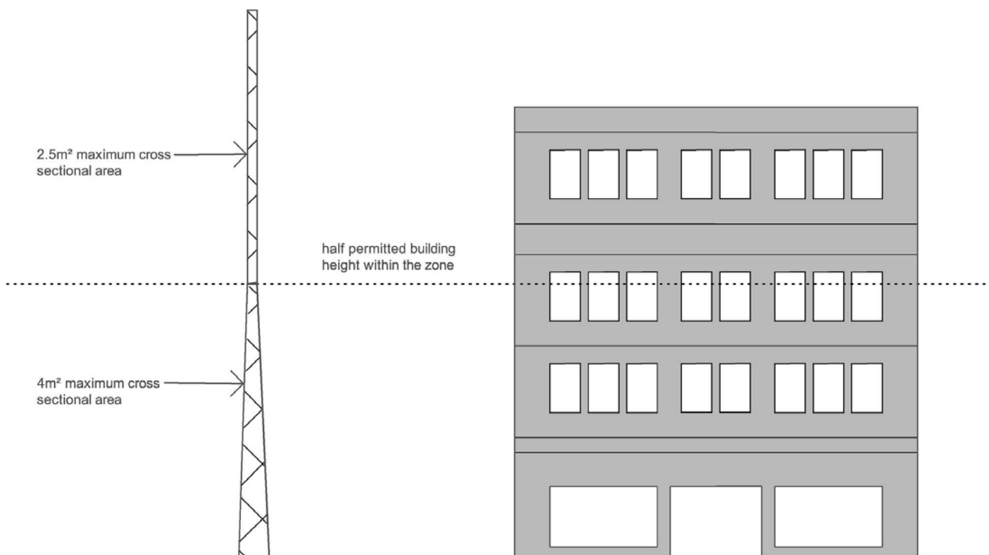
Figure 5.5.3.6B: Cross-sectional area of lattice mast
