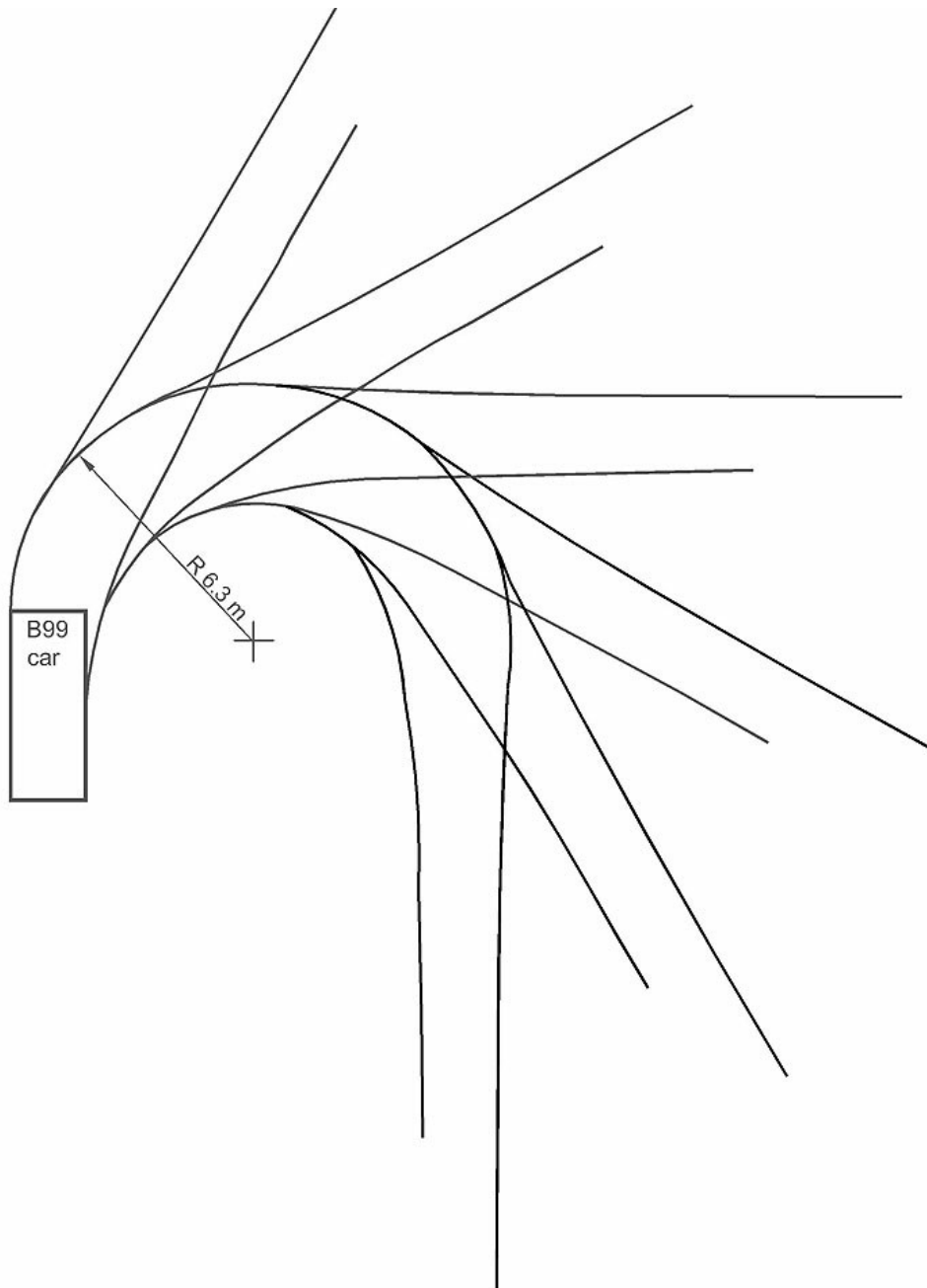
Figure 6B.7 99th percentile vehicle turning circle
