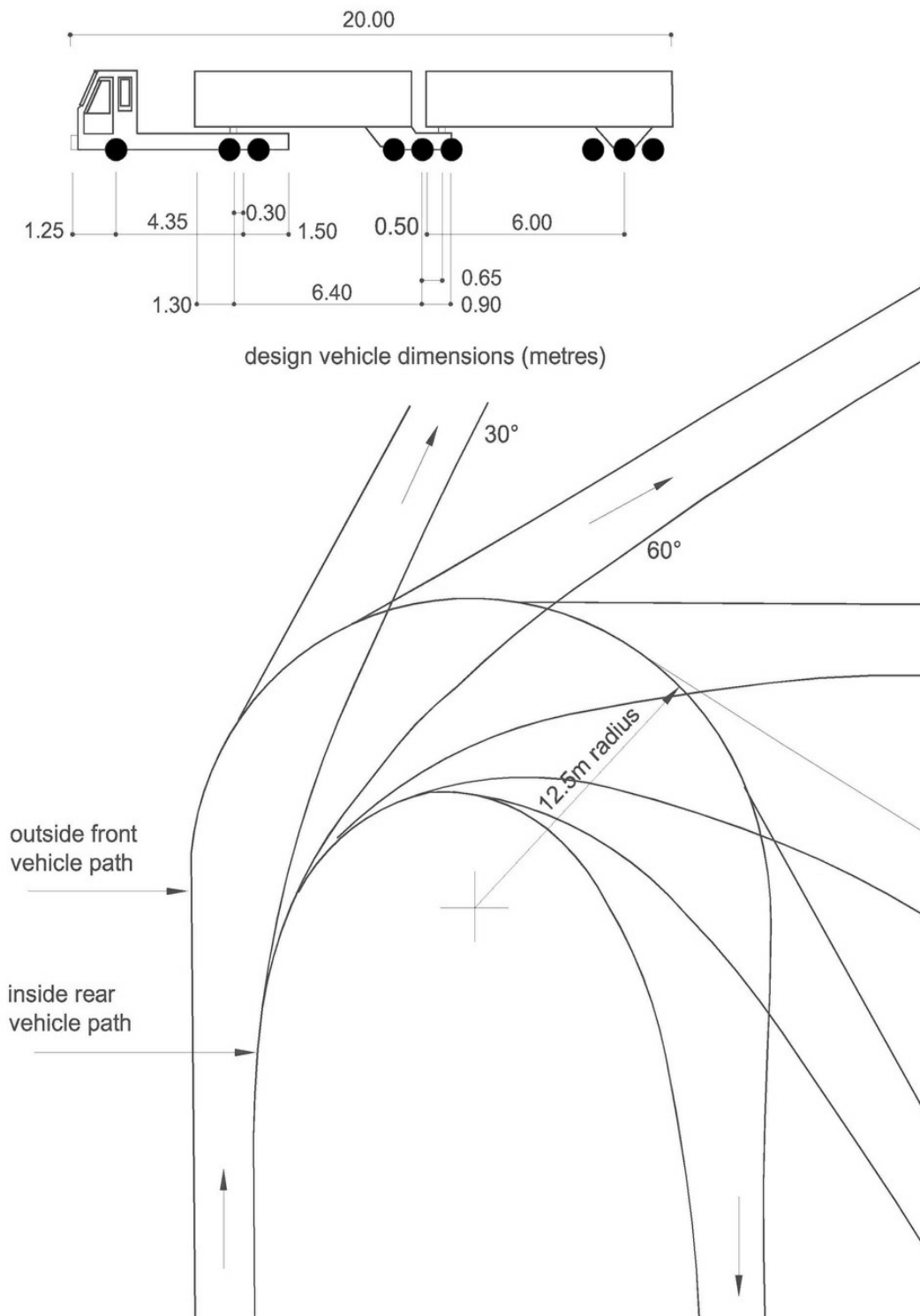
Figure 6B.11 B-train truck turning circle
