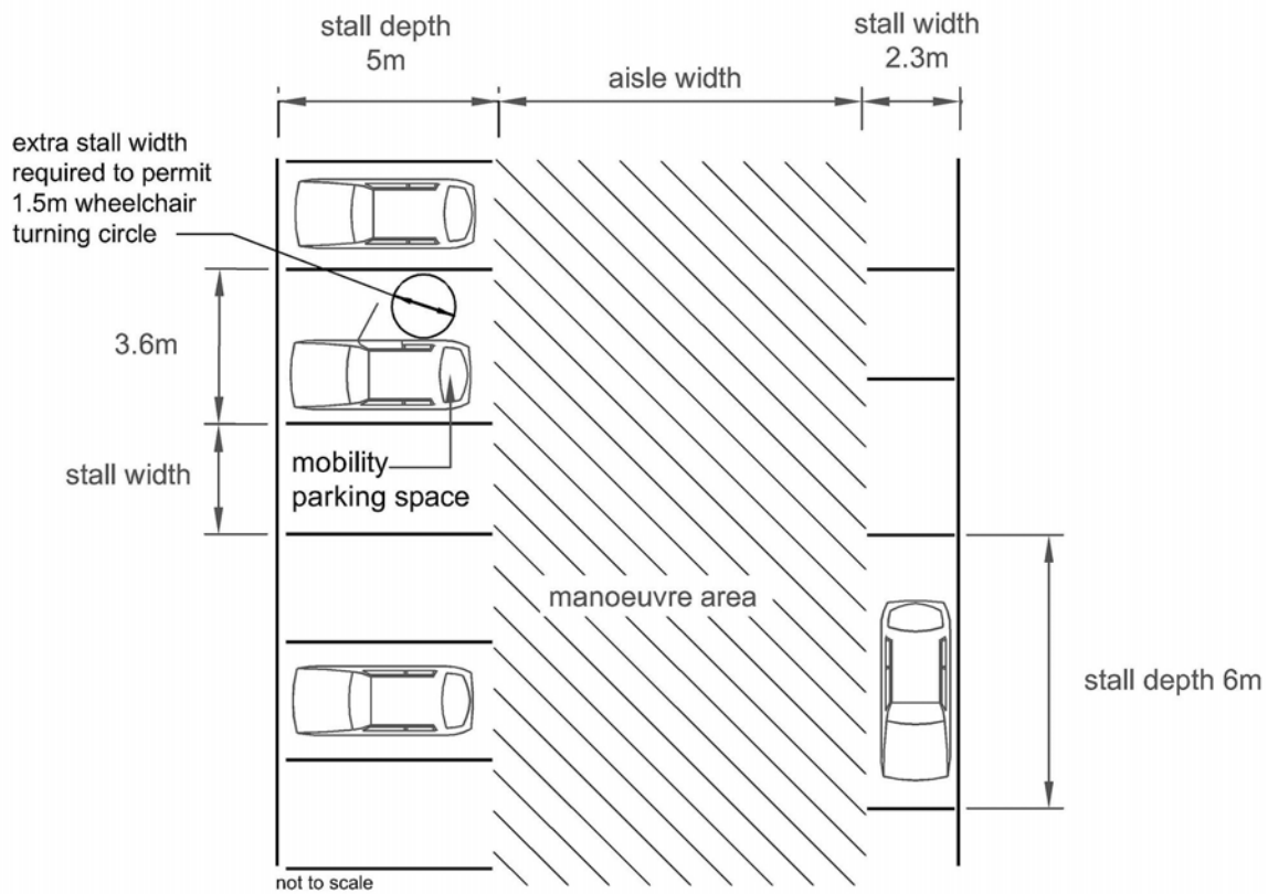
Figure 6B.1 On-site car parking dimensions
