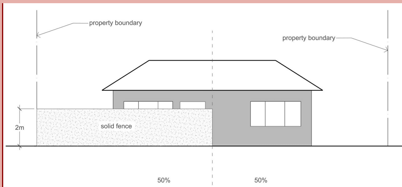
Figure 15.6.2.2A: Examples of fencing that meet Rule 15.6.2.2 Visual Permeability
