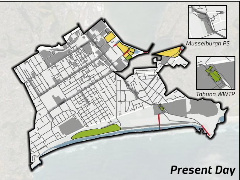
Figure 5.42 Wastewater infrastructure and contaminated land (HAIL sites) risk due to coastal inundation
