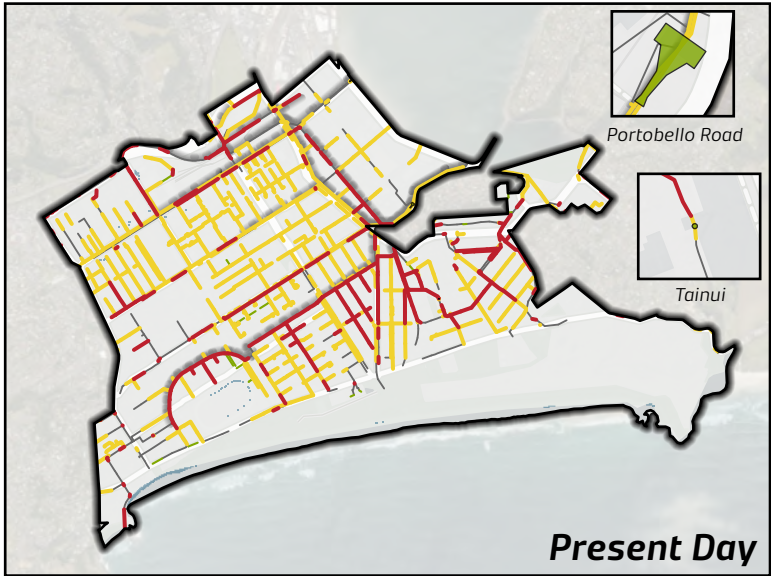
Figure 5.37 Stormwater infrastructure risk due to groundwater
