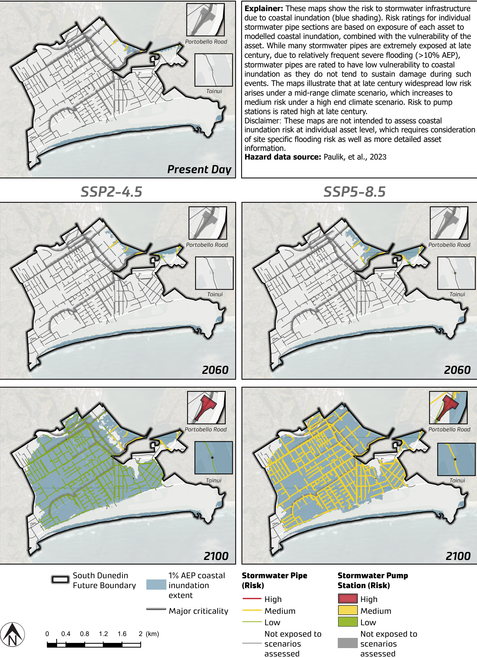
Figure 5.36 Stormwater infrastructure risk due to coastal inundation
