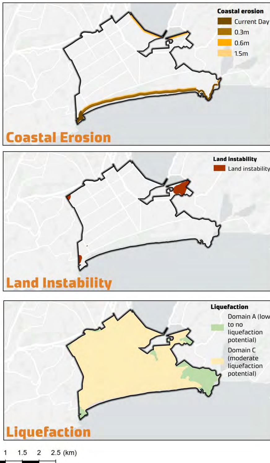
Figure 3.2 Coastal erosion extents (source: (WSP, 2024)), land instability (source: DCC Hazard database data provided for South Dunedin Future programme) and liquefaction (source: (Barrell, 2014) 16
