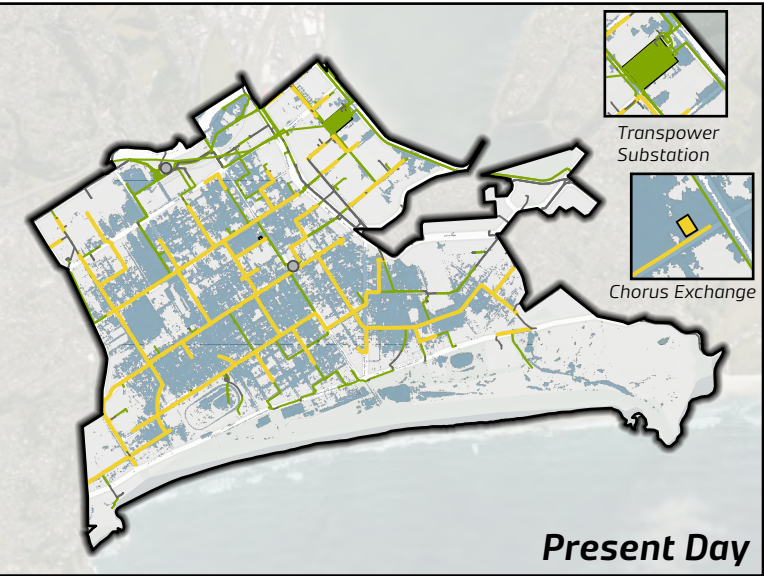
Figure 5.49 Energy and telecommunications infrastructure risk due to pluvial flooding
