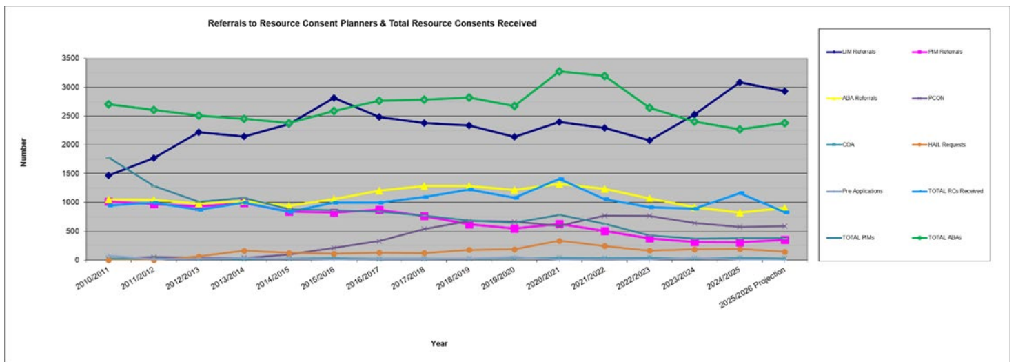
Figure 4: Referral Statistics
