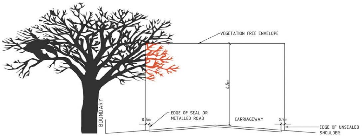
TYPICAL RURAL ROAD CROSS SECTION (SEALED AND UNSEALED WITHOUT WATERTABLES)
