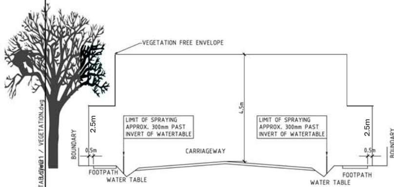
3. TYPICAL URBAN CROSS SECTION (WATER TABLES)
