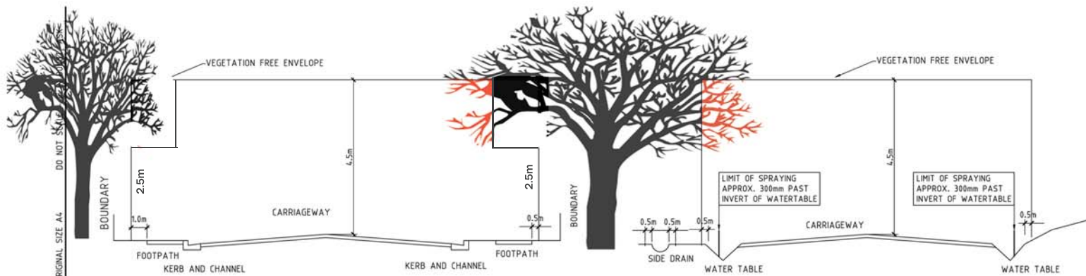
1. TYPICAL URBAN CROSS SECTION (KERB AND CHANNEL)
