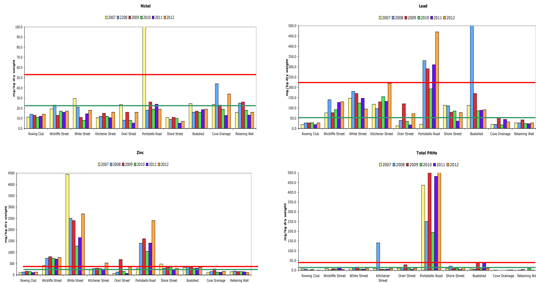
Figure 5 (continued). Graphical representation of contaminant levels in sediment at sampling sites around upper Otago Harbour in 2007, 2008, 2009, 2010, 2011 and 2012. Green line indicates ANZECC low trigger level, red line is high trigger level.
