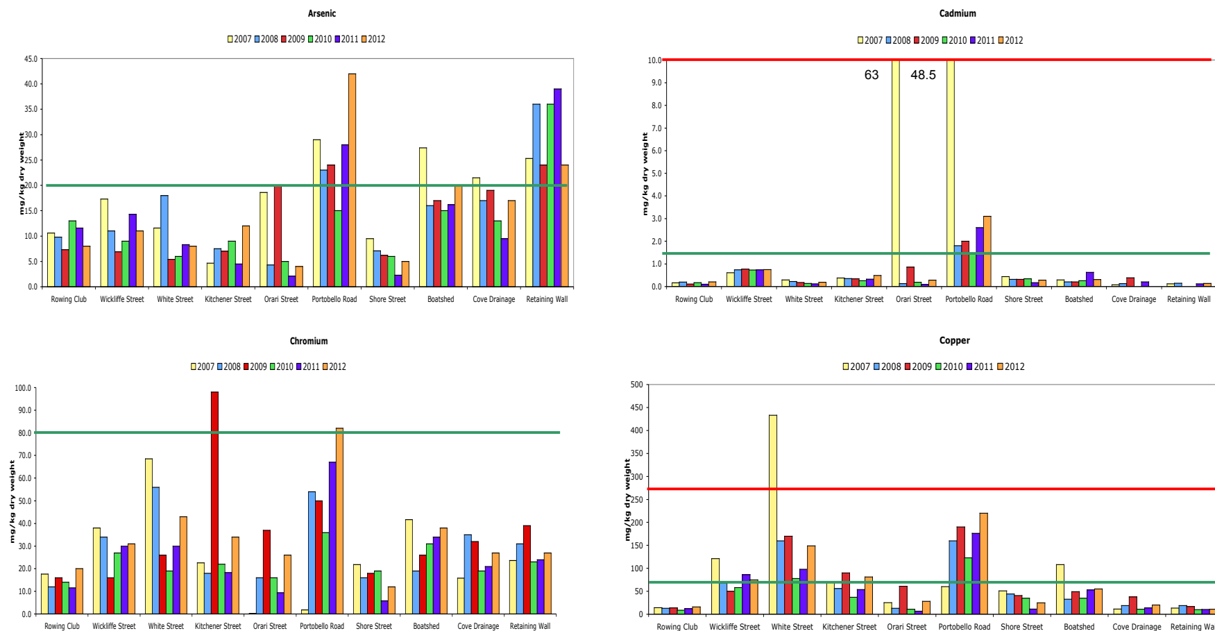
Figure 5. Graphical representation of contaminant levels in sediment at sampling sites around upper Otago Harbour in 2007, 2008, 2009, 2010, 2011 and 2012. Green line indicates ANZECC low trigger level, red line is high trigger level.
