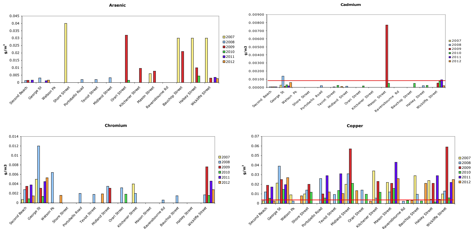
Figure 4. Graphical representation of contaminant levels in stormwater at outfalls around upper Otago Harbour in 2007, 2008, 2009, 2010, 2011 and 2012. Red line indicates ANZECC trigger level for protection of 80% of species.
